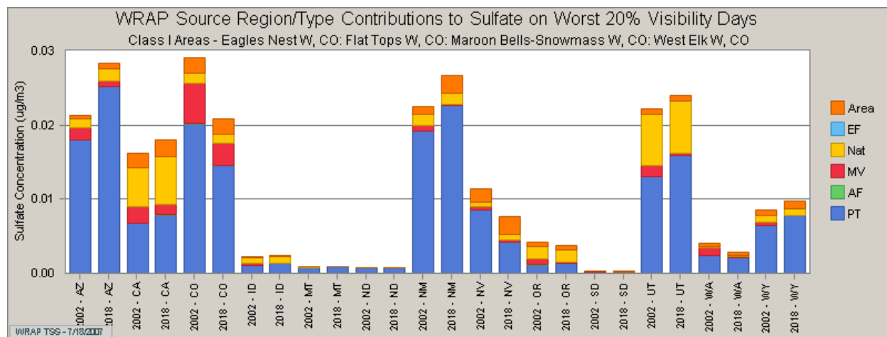
Figure 7-1: Sulfate PSAT - Source Region Bar Chart for Worst Days in 2002 and 2018
