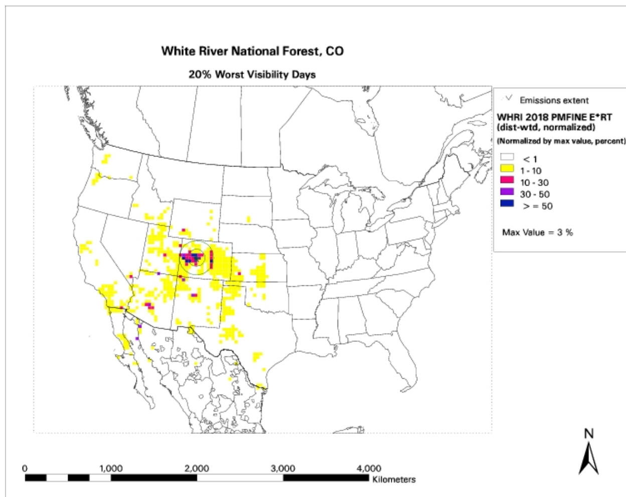
Figure 5-23: Regional PM Fine WEP for 2018 Worst Days
