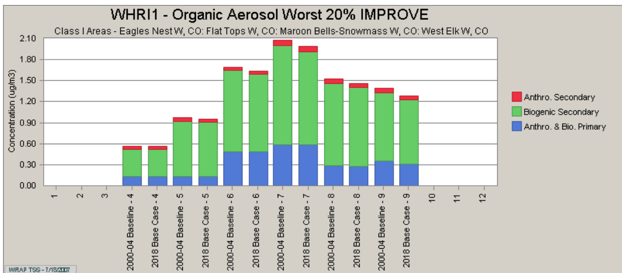
Figure 7-9: Organic Carbon PSAT - Bar Chart for Worst Days in 2002 and 2018
