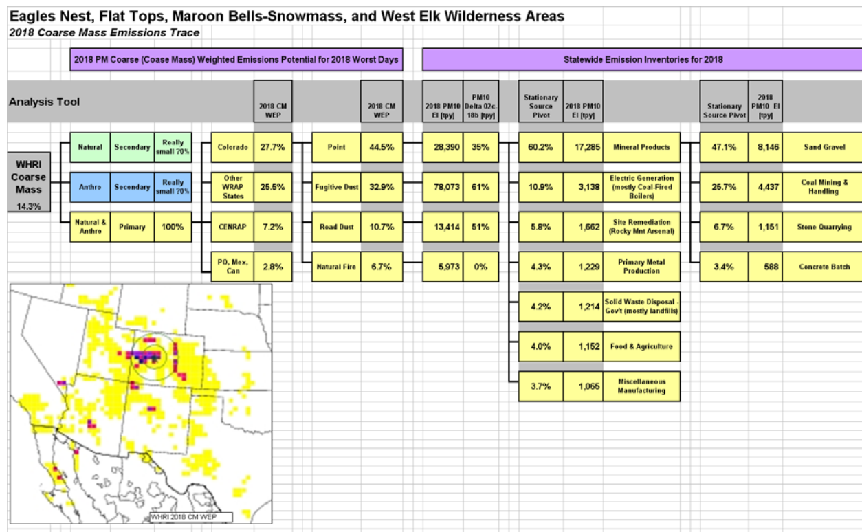
Figure 8-6: Coarse Mass Emissions Trace for 2018 Worst Days
