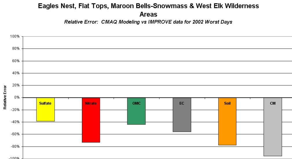
Figure 6-2: Relative Error: CMAQ Model vs IMPROVE data for WHRI 2002 Worst Days
