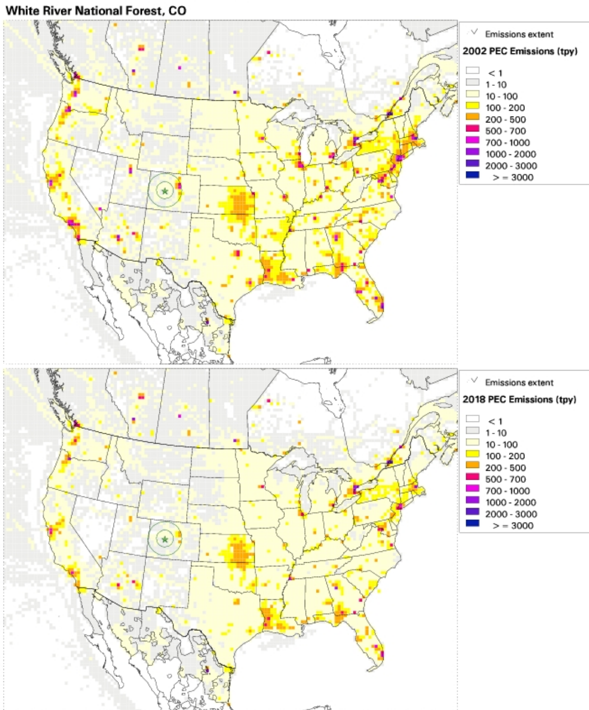
Figure 5-10: Regional EC Emissions – 2002& 2018 Inventory
