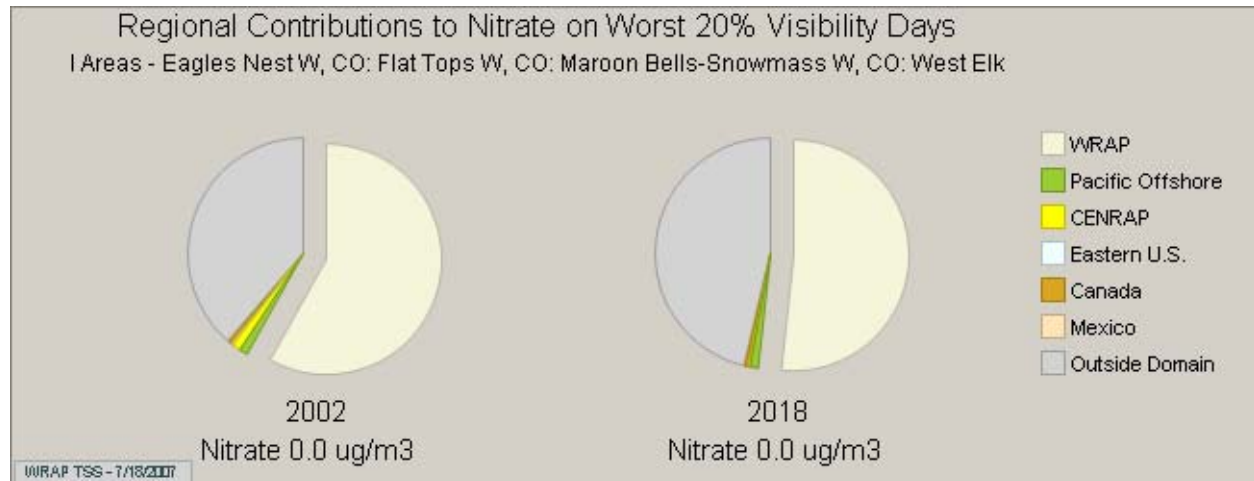
Figure 7-6: Nitrate PSAT - Regional Pie Chart for Worst Days in 2002 and 2018
