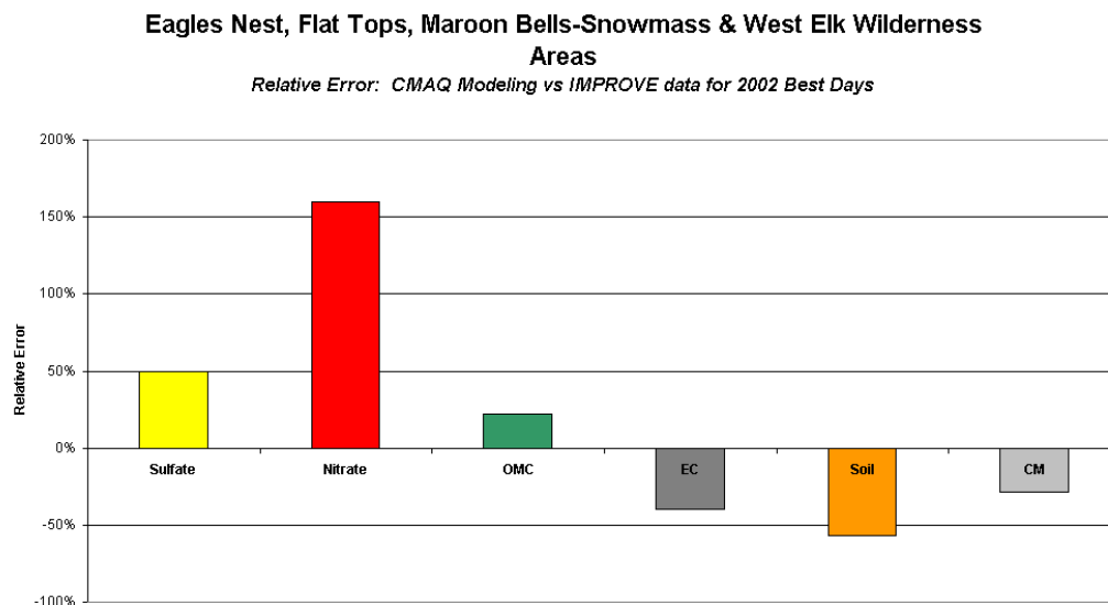
Figure 6-4: Relative Error: CMAQ Model vs IMPROVE data for WHRI 2002 Best Days
