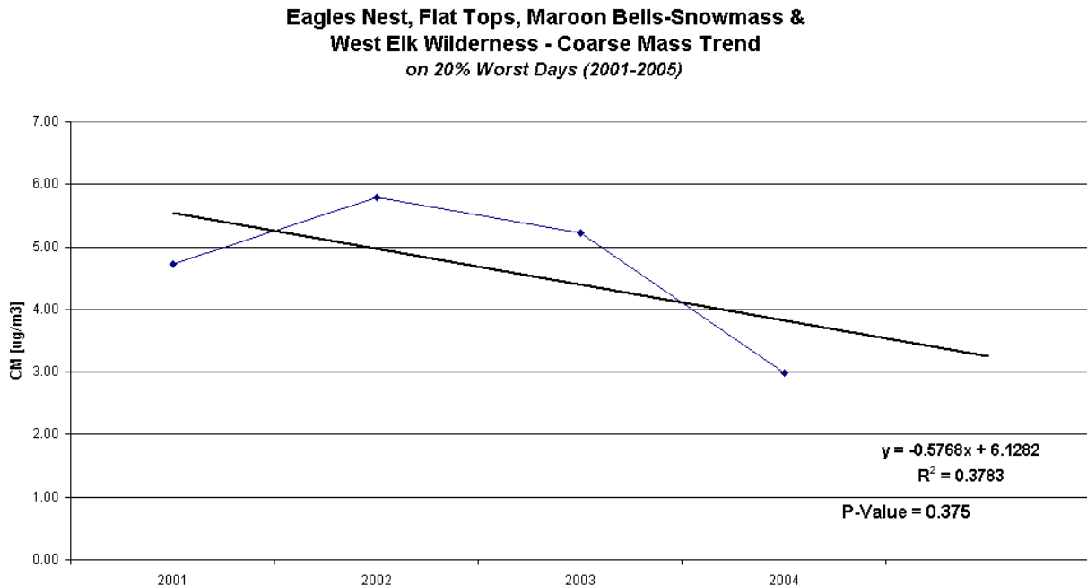
Figure G -6: Coarse Mass Trend
