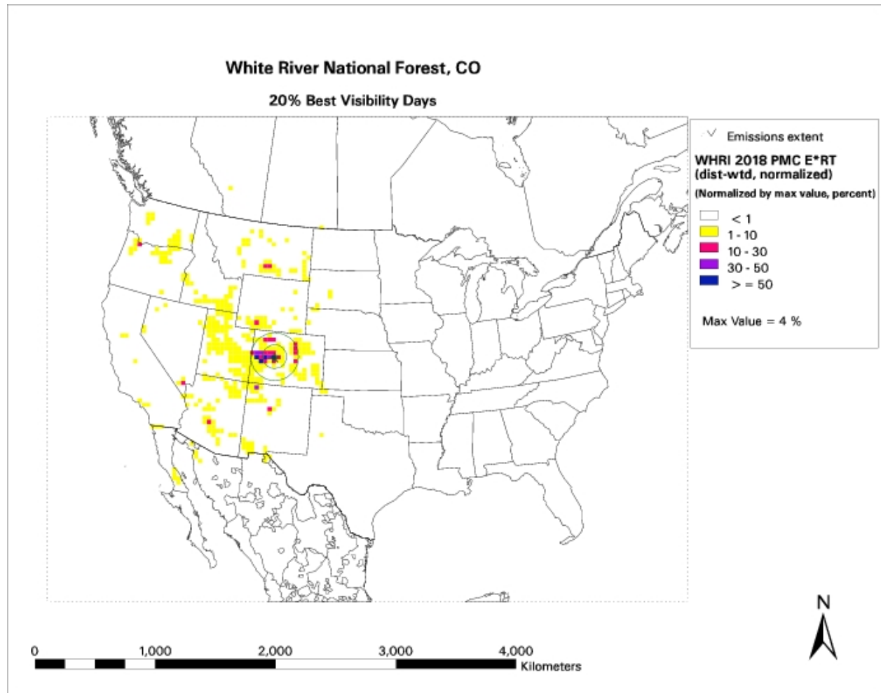
Figure 5-26: Regional PMC WEP for 2018 Best Days
