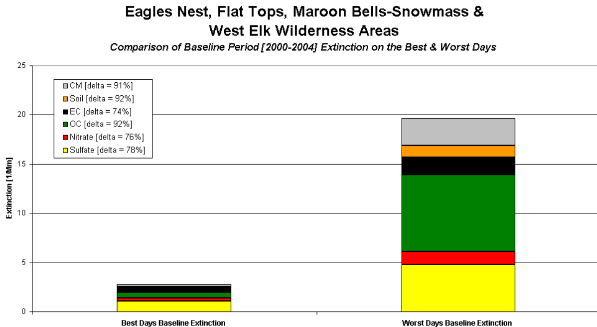
Figure 4-5: Comparison of Baseline Extinction for 20% Best & Worst Days
