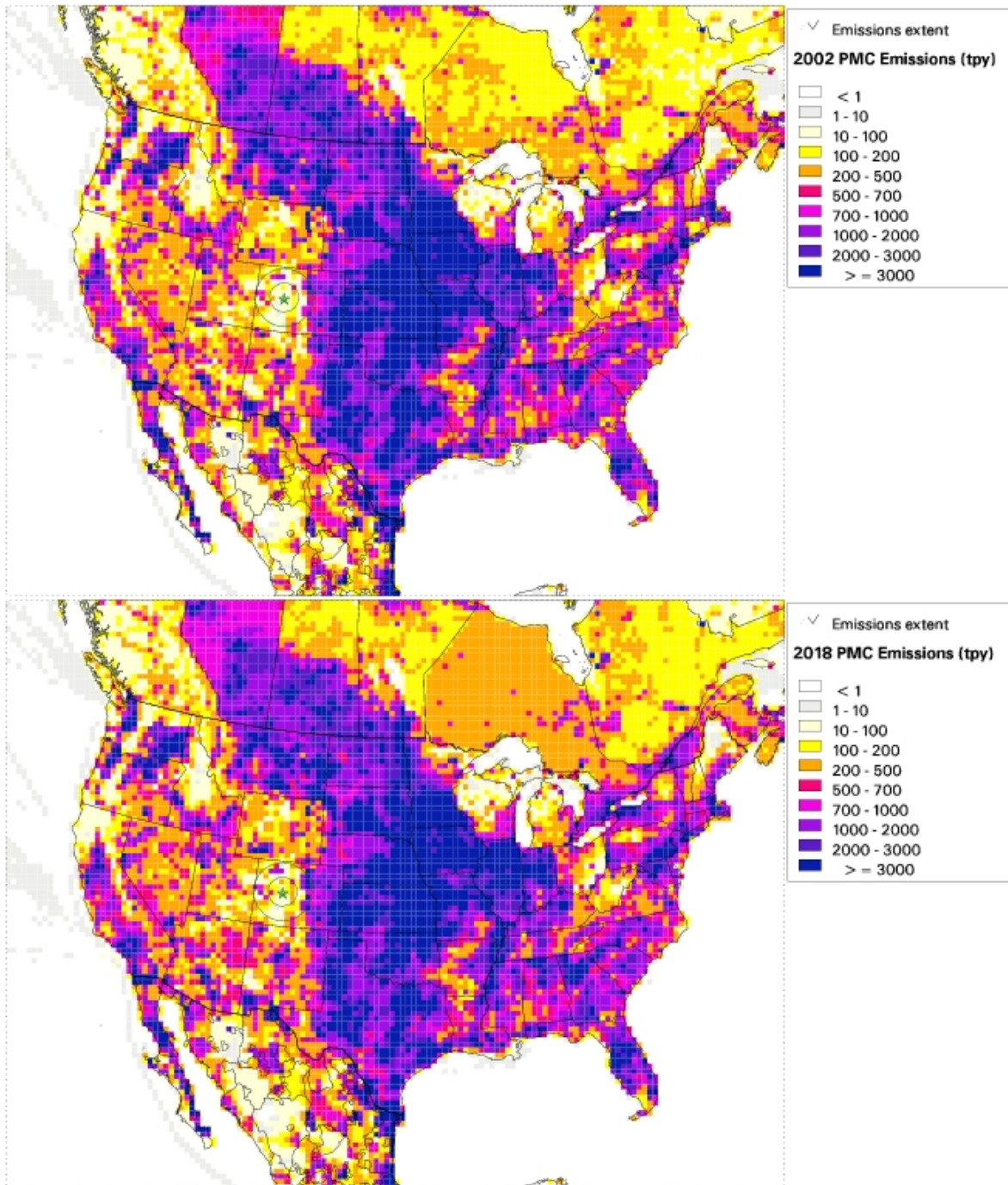
Figure 5-14: Regional PMC Emissions – 2002 & 2018 Inventory
