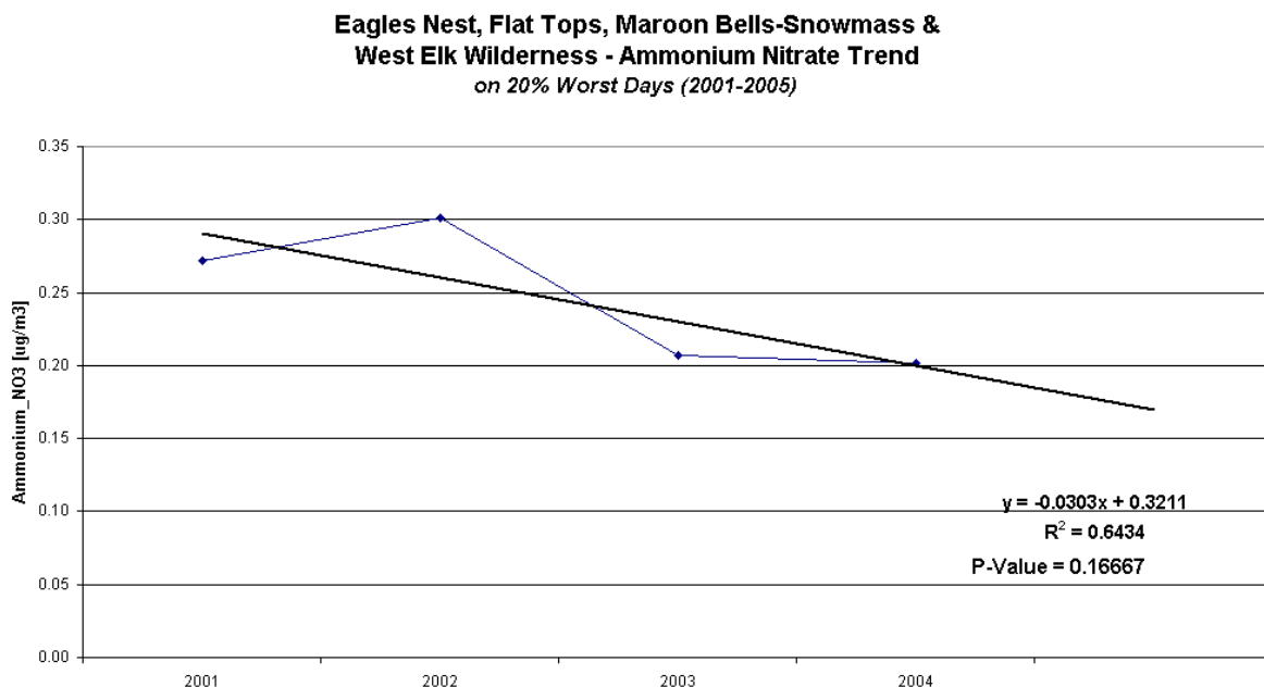
Figure G -2: Ammonium Nitrate Trend
