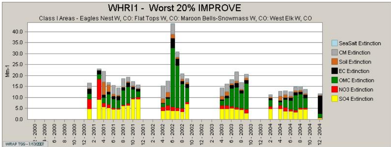
Figure 4-7: Monthly Distribution of 20% Worst Days
