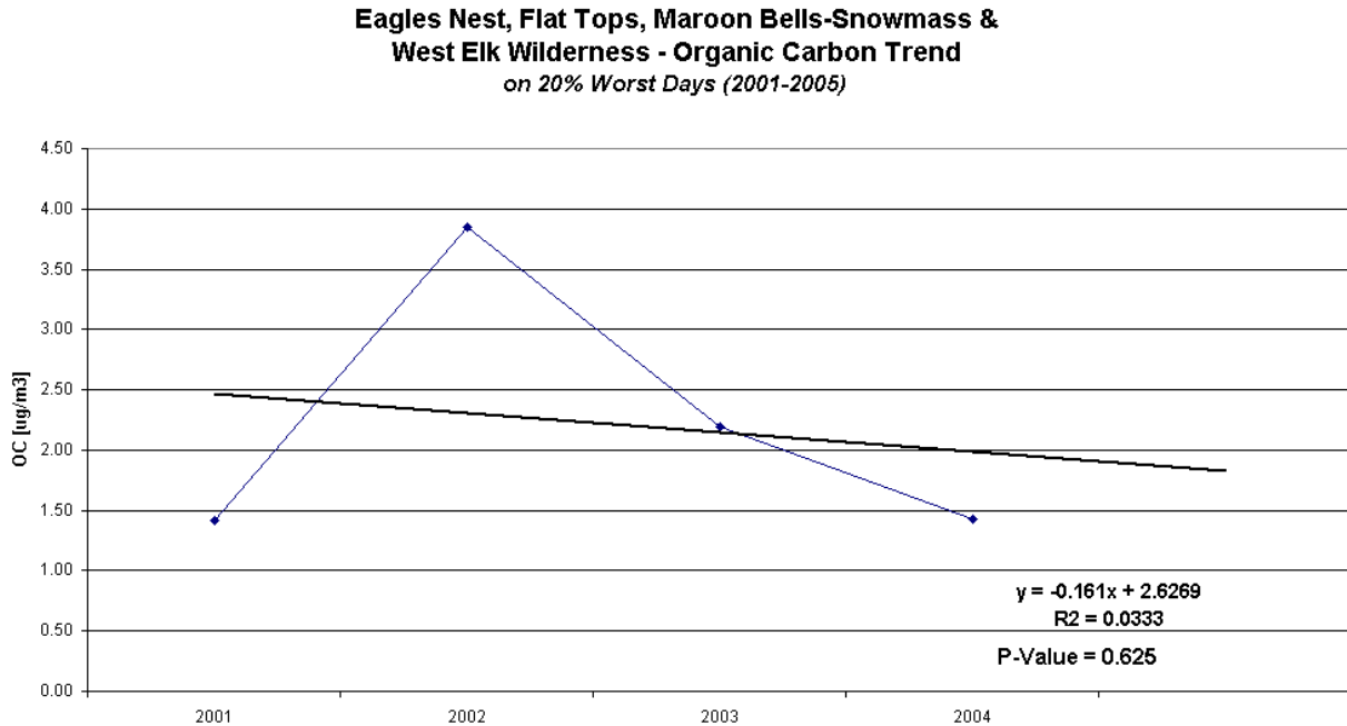
Figure G -3: Organic Carbon Trend
