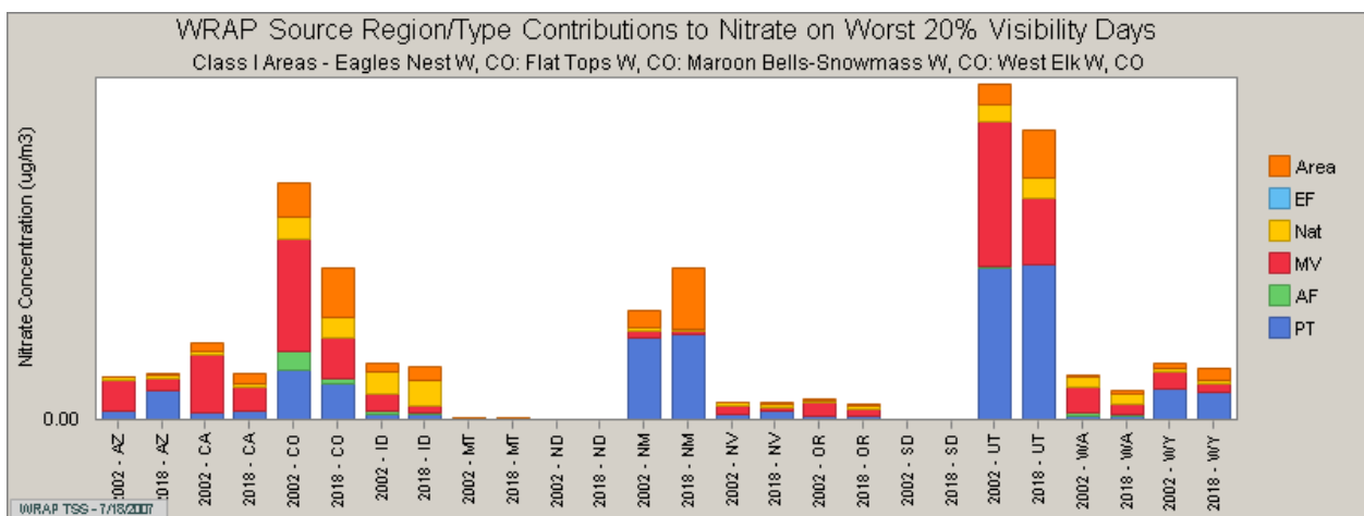
Figure 7-5: Nitrate PSAT – Source Region Bar Chart for Worst Days in 2002 and 2018
