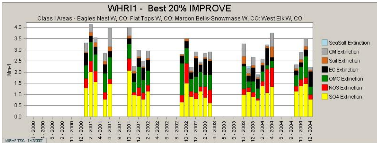
Figure 4-8: Monthly Distribution of 20% Best Days
