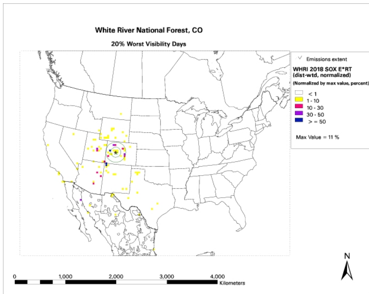
Figure 5-15: Regional SO x WEP for 2018 Worst Days
