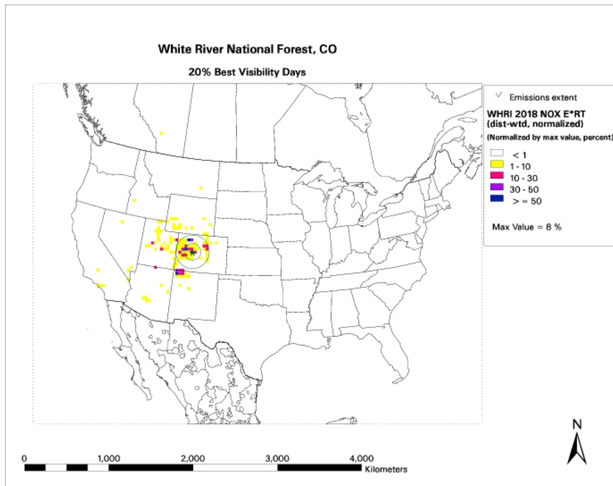
Figure 5-18: Regional NO x WEP for 2018 Best Days
