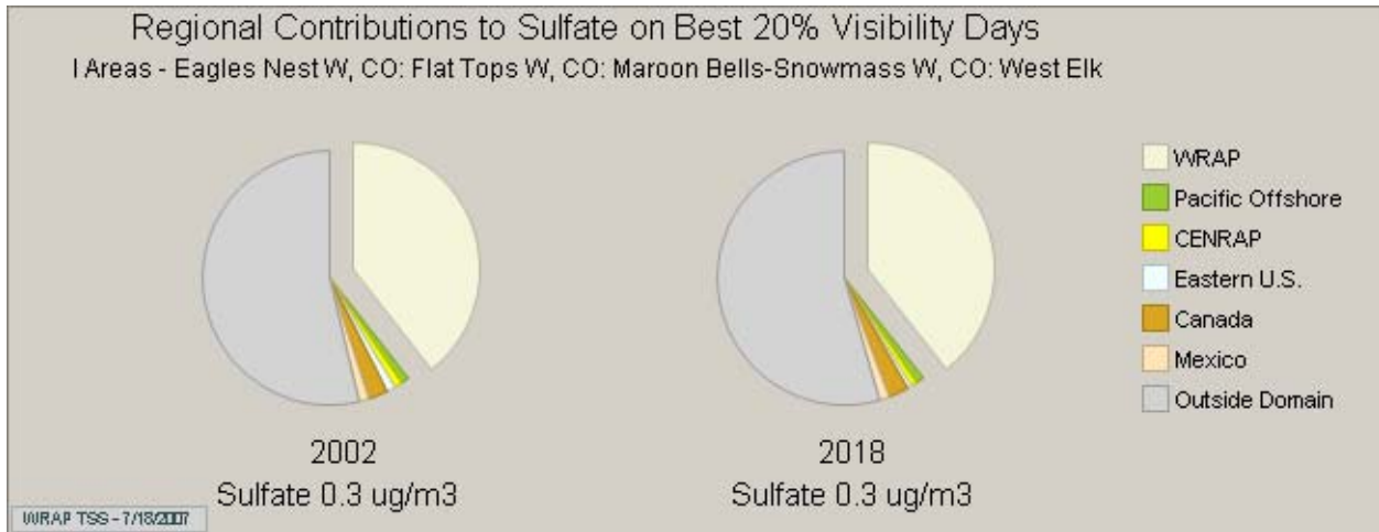
Figure 7-4: Sulfate PSAT - Regional Pie Chart for Best Days in 2002 and 2018
