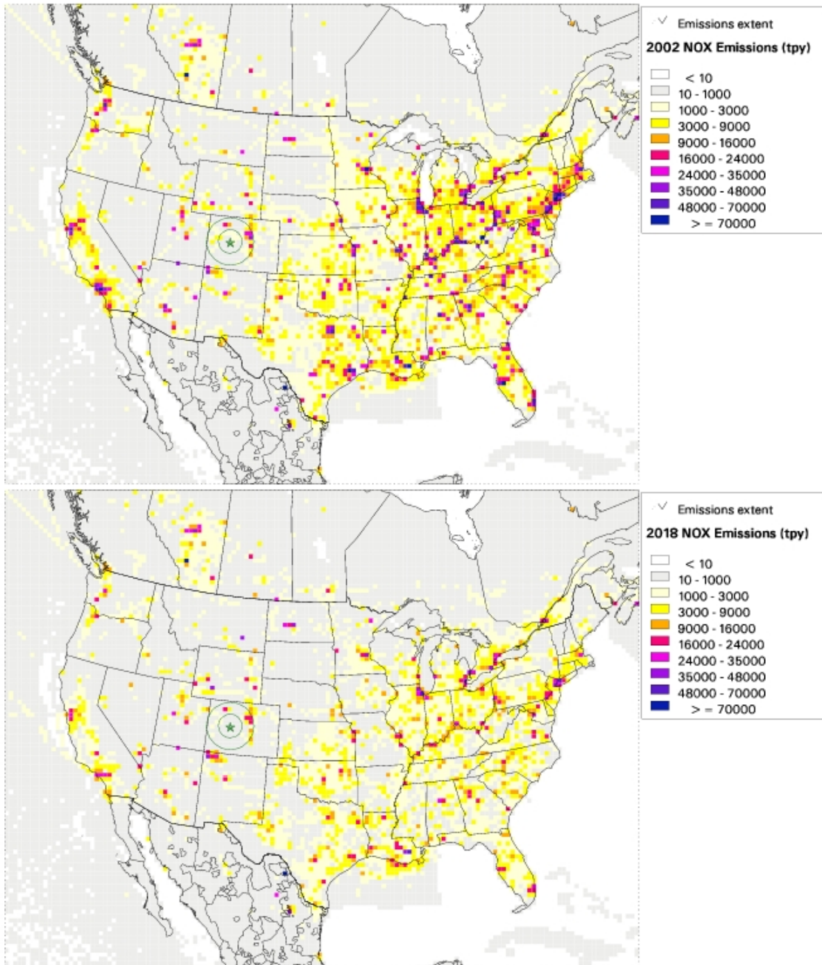
Figure 5-4: Regional NOx Emissions – 2002 & 2018 Inventory
