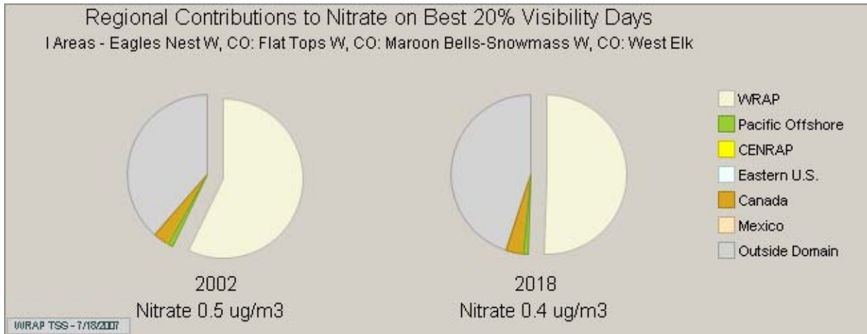
Figure 7-8: Nitrate PSAT - Regional Pie Chart for Best Days in 2002 and 2018
