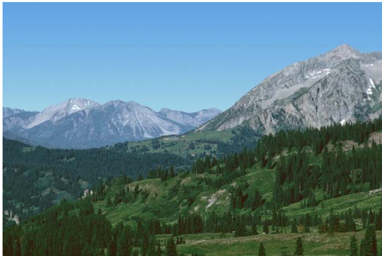
Figure 3-1: West Elk Wilderness - Baseline Best Days
