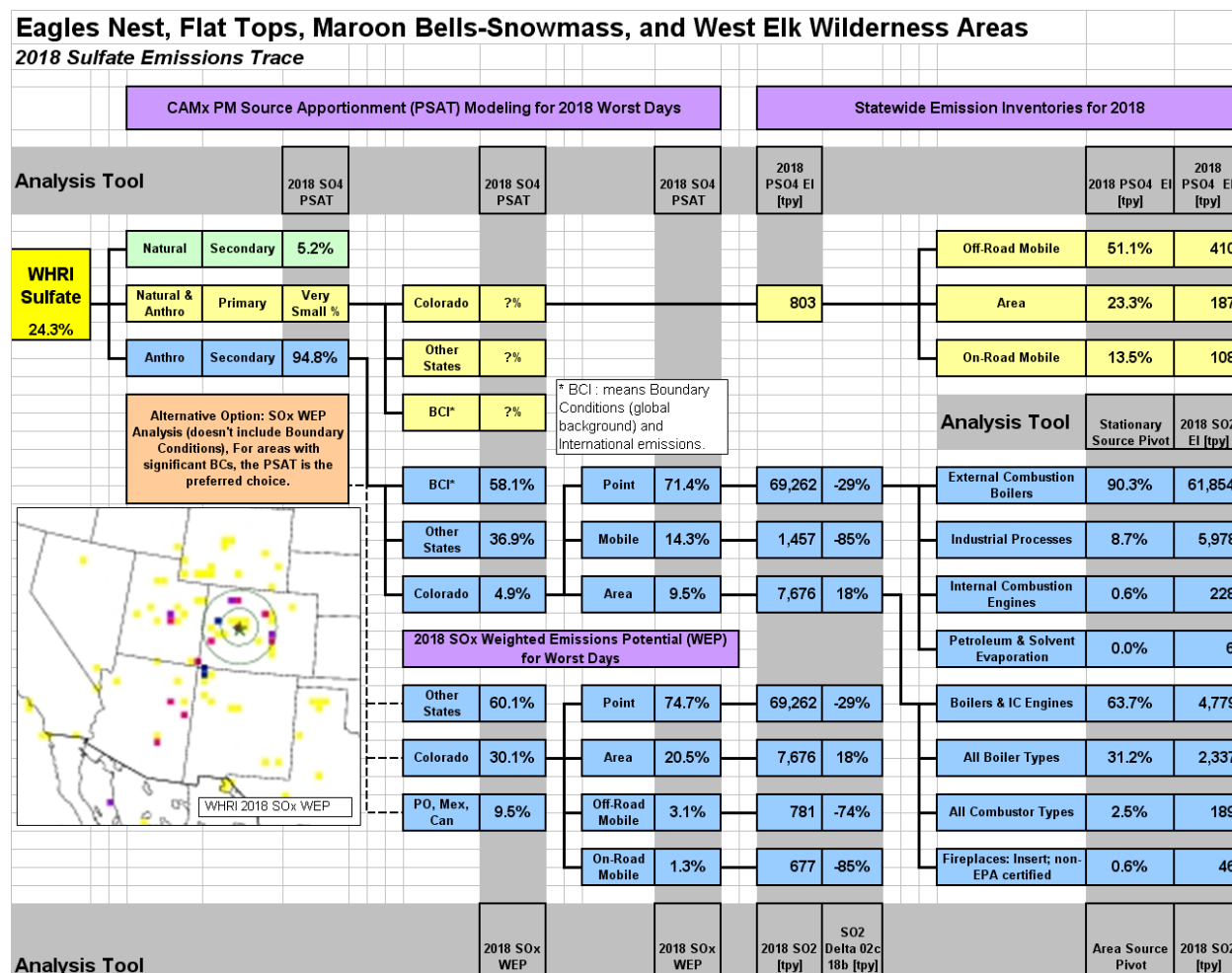
Figure 8-1: Sulfate Emissions Trace for 2018 Worst Days
