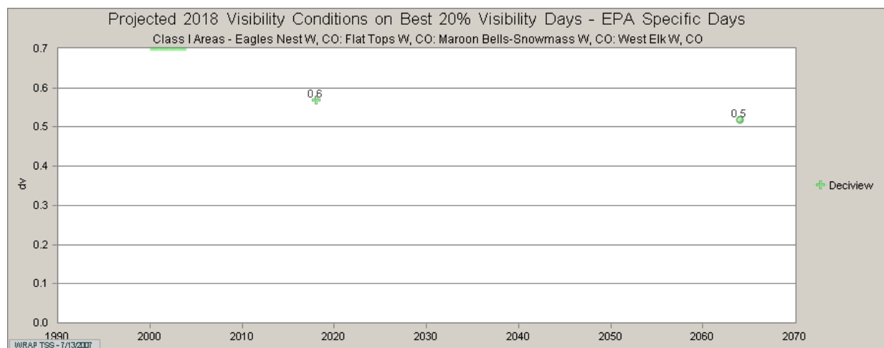
Figure 6-8: CMAQ Model Projections in Haze Index for WHRI 2018 Worst Days
