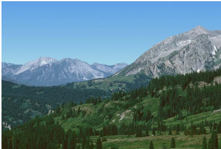
Figure 3-3: West Elk Wilderness - Natural Best Days
