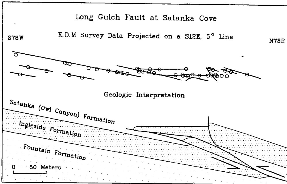
Figure 10. Down-plunge projection of Long Gulch fault Satanka Cove.
