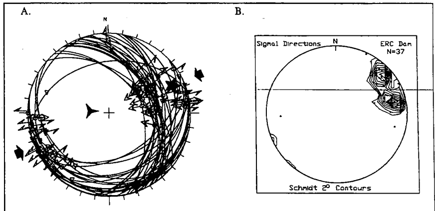
Figure 9. Paleostress analysis of slickensides seen at Stop 3 using A) the direct stress inversion method of Angelier (1990) and B) Schmidt contours of the ideal \sigma_1 direction method of Compton (1966).
