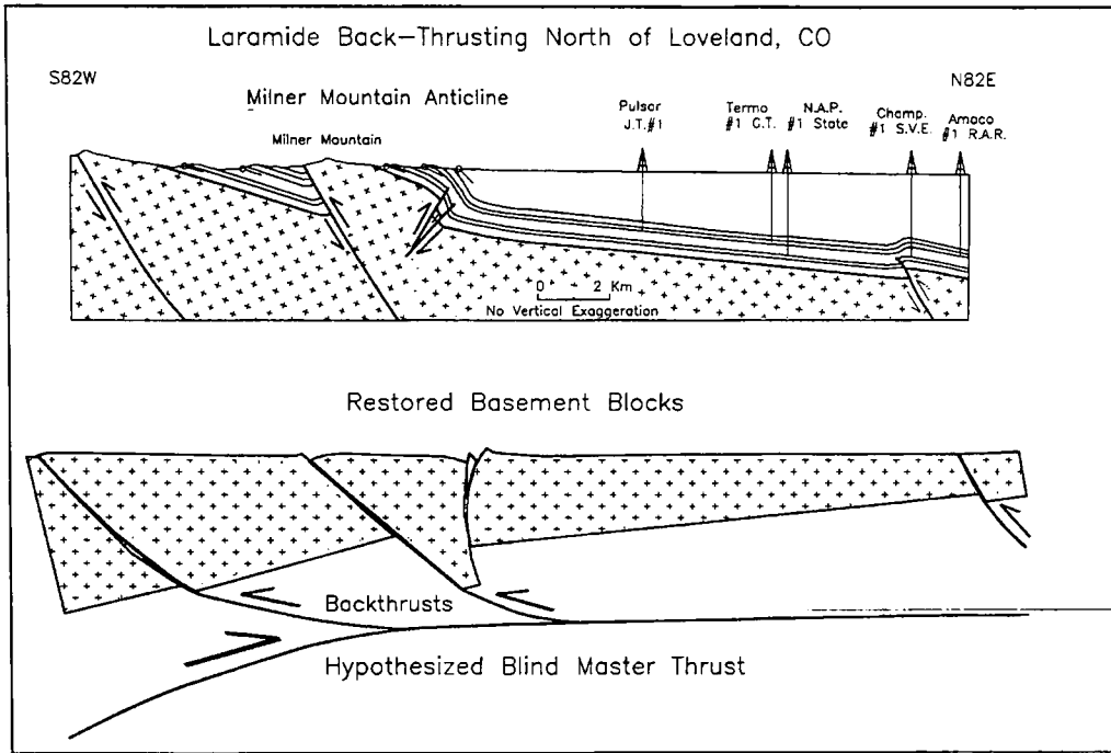
Figure 8. Blind master thrust hypothesis explains reversed thrusting along the eastern margin of the northern Front Range.
