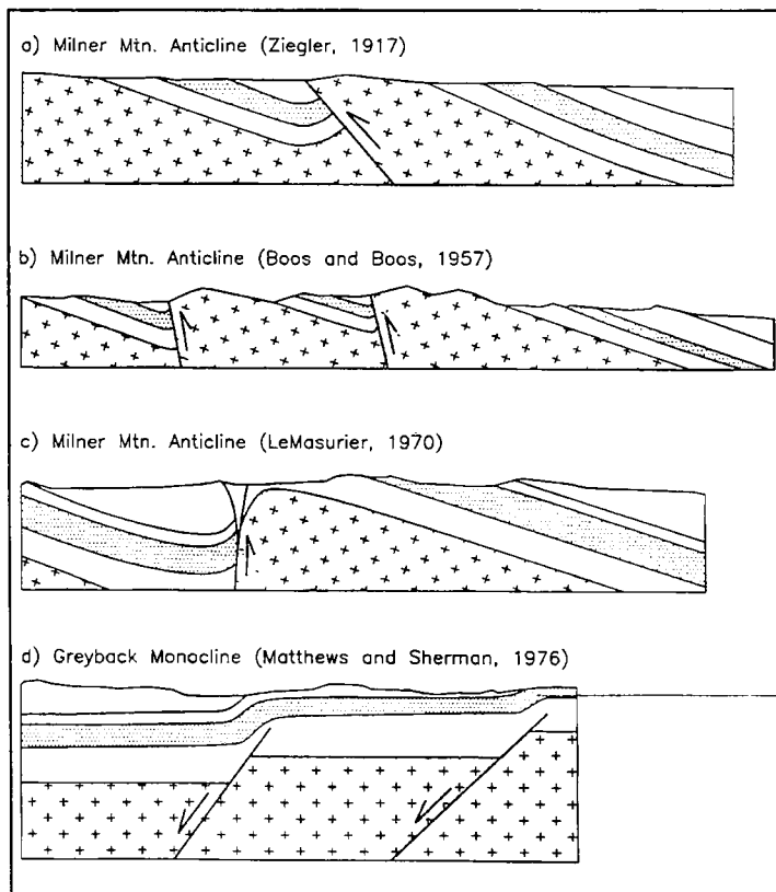
Figure 2. Evolution of structural interpretations through time as discussed in text.
