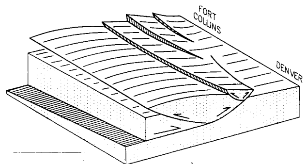
Figure 12. Block diagram of the transitional thrust structure along the Denver basin margin with the northeastern Front Range.
