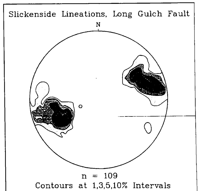
Figure 11. Lower hemisphere projection of slickenside lineations adjacent to the Long Gulch fault exposed in Satanka Cove.
