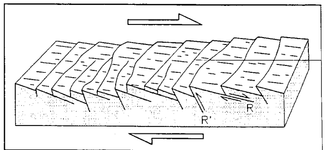
Figure 4. Diagram of a striated fault surface illustrating the stepped Riedel shear morphology (after Petit, 1987; Allmendinger et al., 1989; Gregson 1994).
