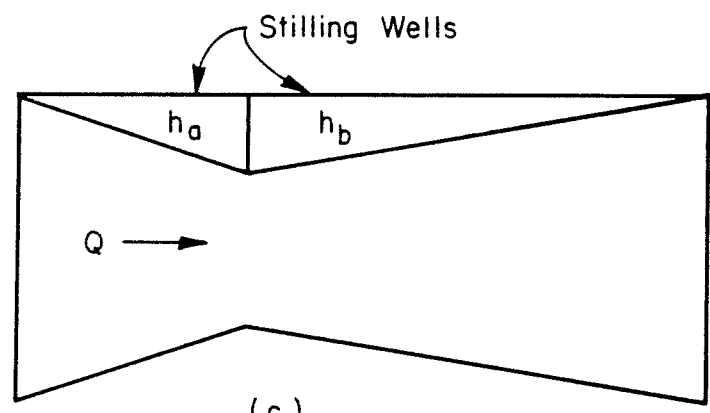
Figure 9. Plan view of Cutthroat flume showing various methods of constructing stilling wells.
