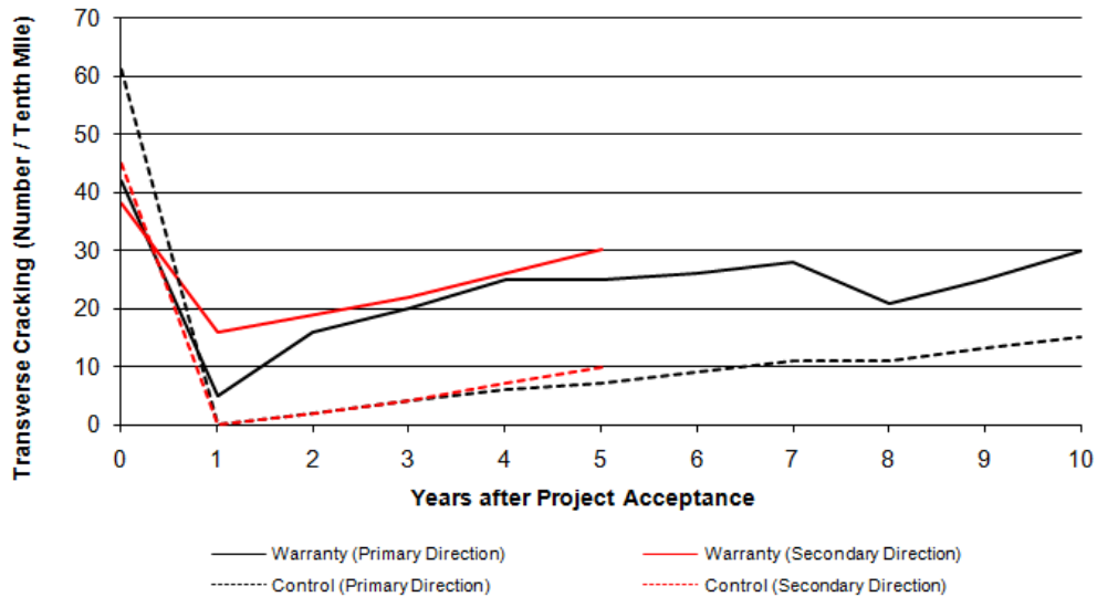
Figure 68. Comparison of US 36 East of Byers/US 36 West of Byers transverse cracking performance
