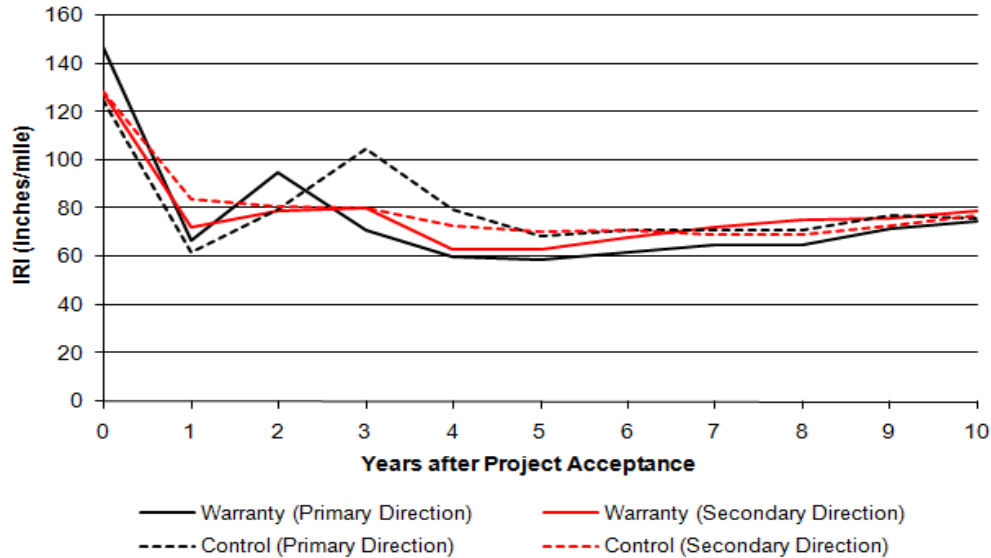
Figure 28. Comparison of I-25 N. of Pueblo / I-25 Young Hollow IRI performance
