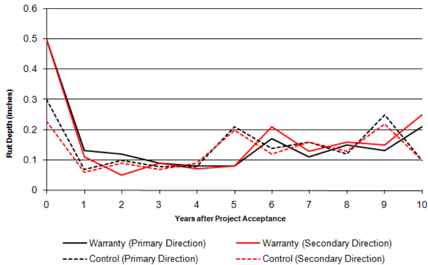
Figure 8. Comparison of the I-25 Fountain / I-25 Pueblo rut depth performance
