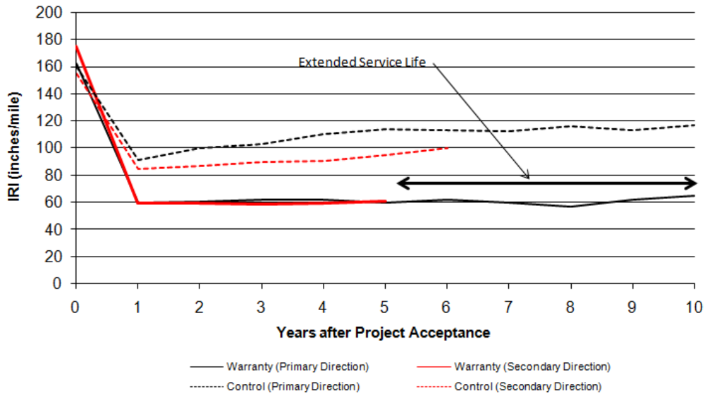
Figure 70. Comparison of the US 287 / SH 119 IRI performance
