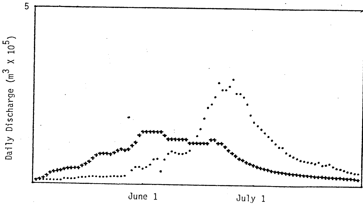
Figure 6.7. Observed (·) and Simulated (+) Hydrographs for Darling Creek (WY 1971).
