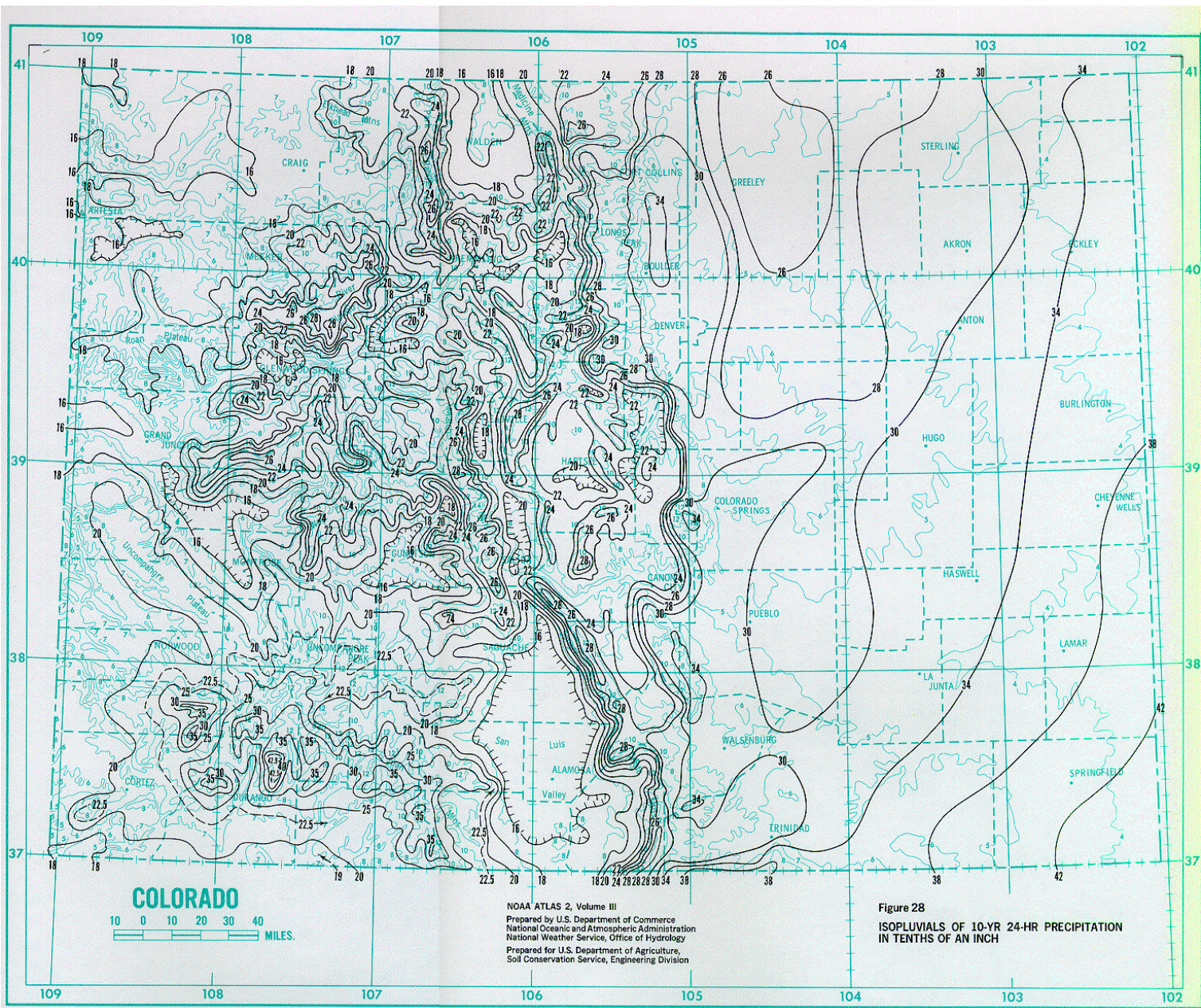
Figure 2.3 Isopluvials of 10-year 24-hour precipitation in tenths of an inch for the State of Colorado.
