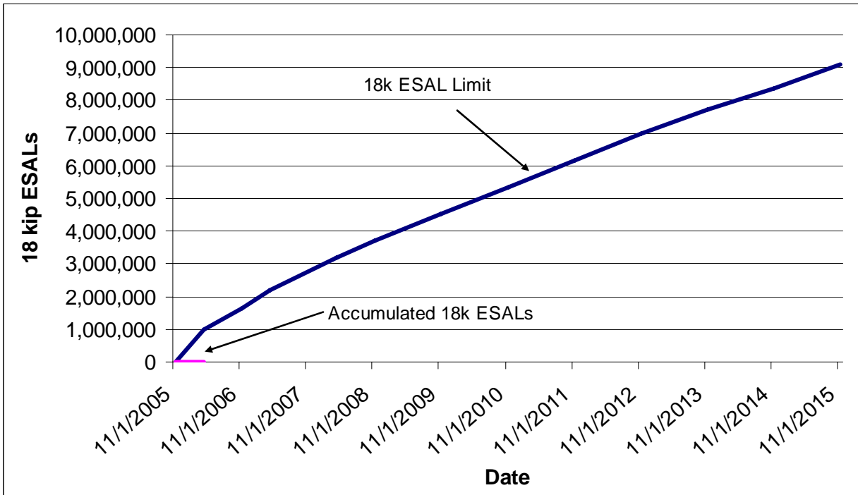
Figure 9. Accumulated traffic load on the Constitution Ave. to Garrett Rd. project.
