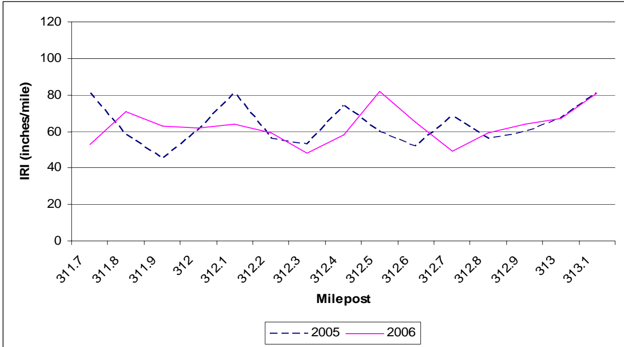
Figure 7a. PMS data for International Roughness Index on the SH 94 to Constitution Ave. project (control).
