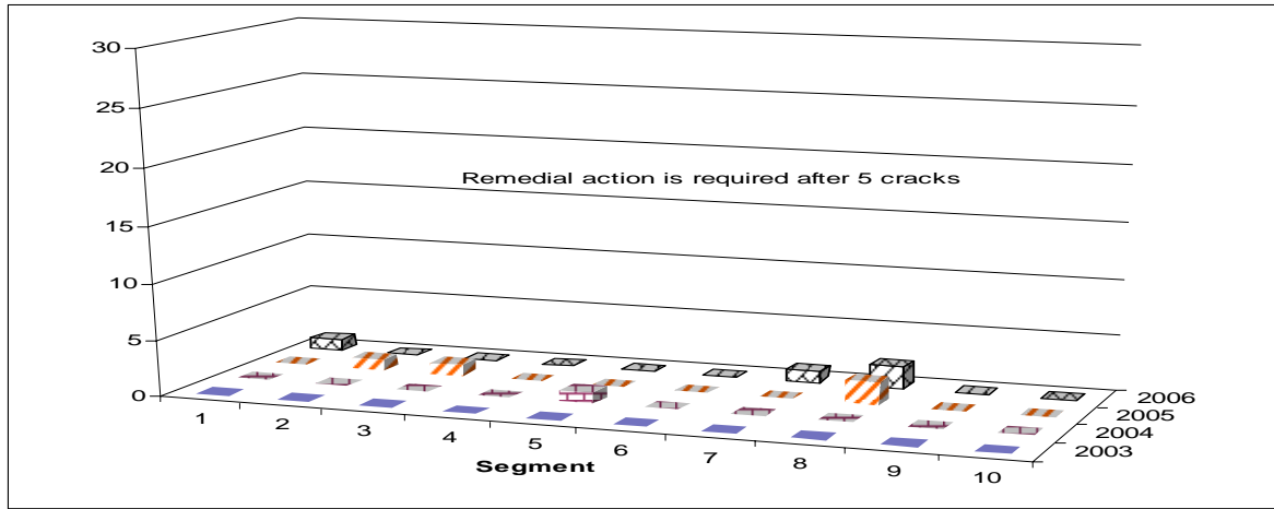
Figure 3c. PMS data for transverse cracks in the secondary direction on the Stratton project (warranty).
