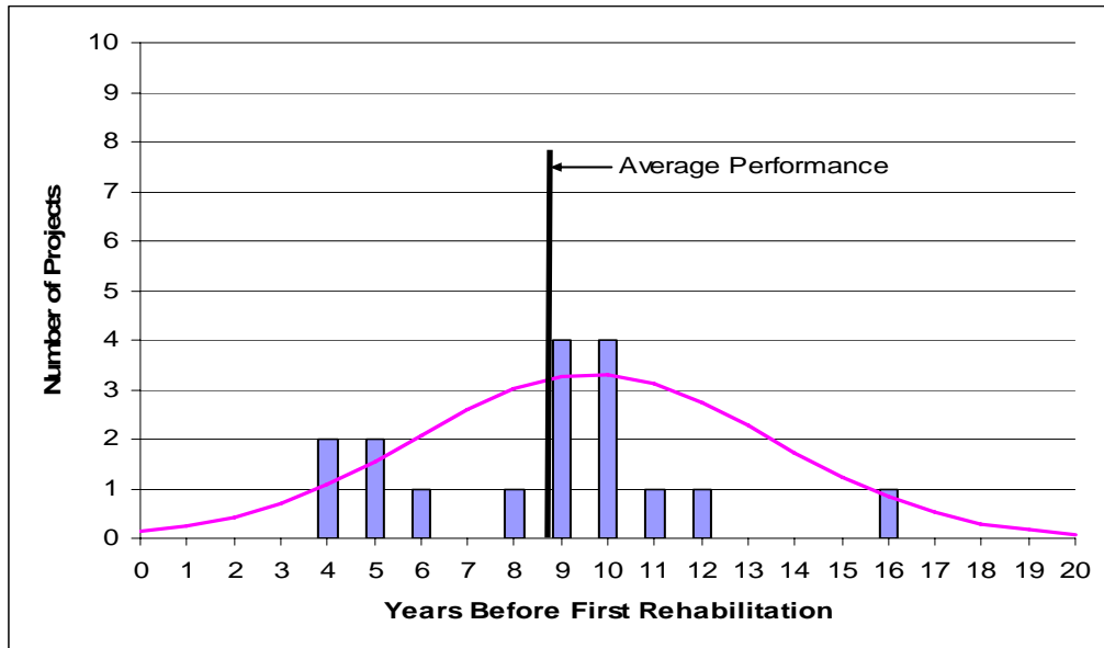
Figure 1. Historical performance of 32 HMA paving projects with 20-year design life.
