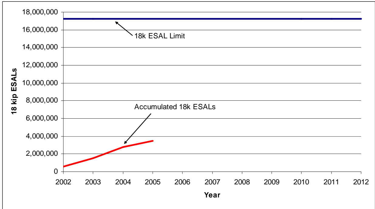
Figure 6. Accumulated traffic load on the Stratton project.
