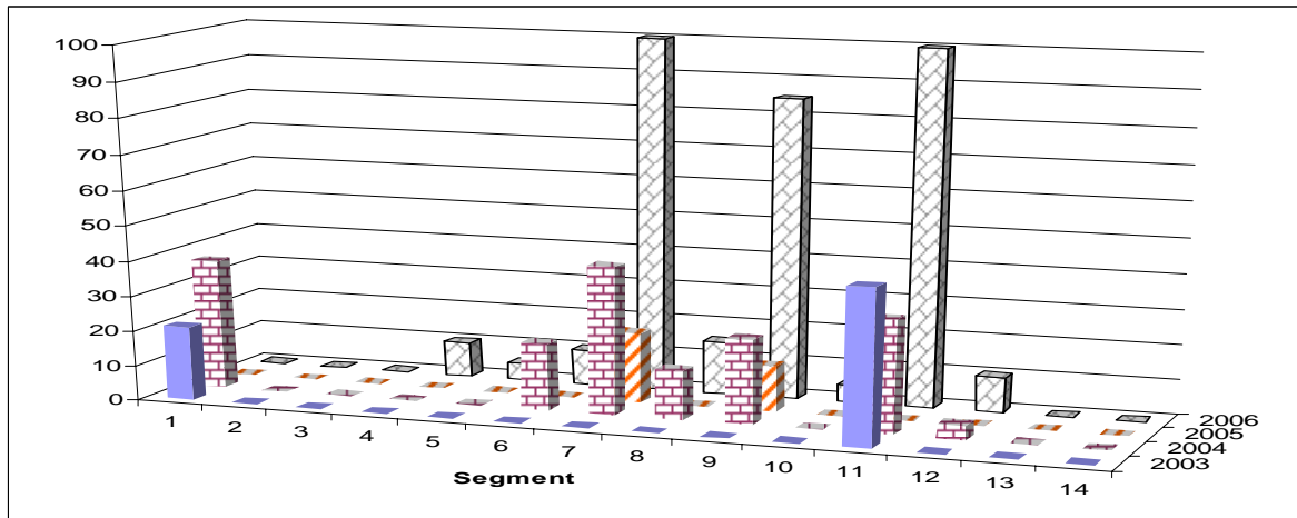
Figure 4a. PMS data for longitudinal cracks on the Eads project (control).
