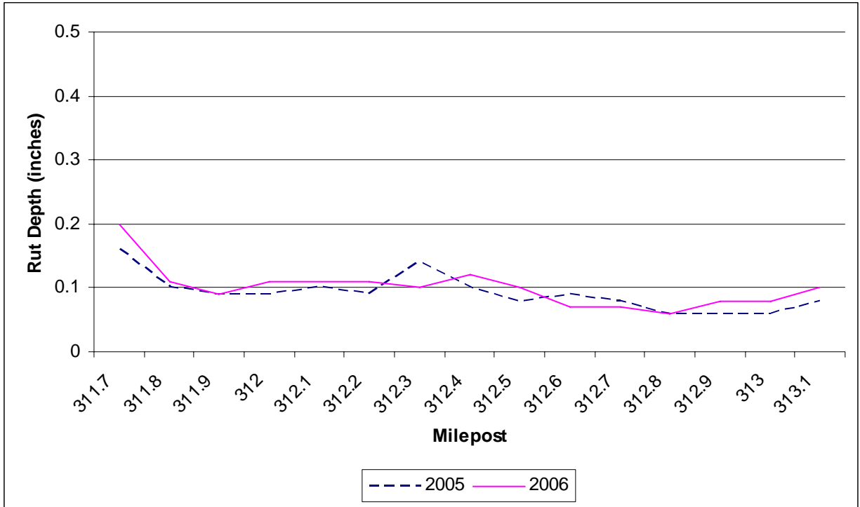
Figure 8a. PMS data for rutting on the SH 94 to Constitution Ave. project (control).
