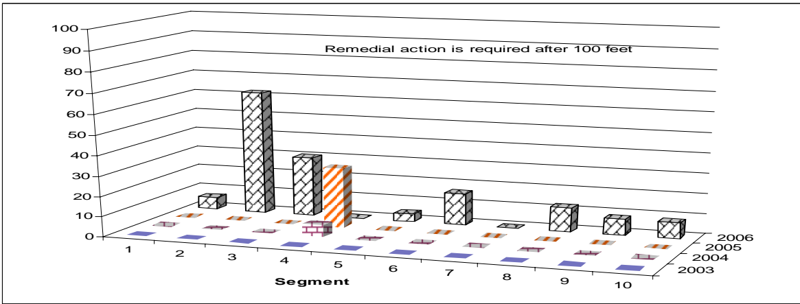
Figure 4c. PMS data for longitudinal cracks in the secondary direction on the Stratton project (warranty).
