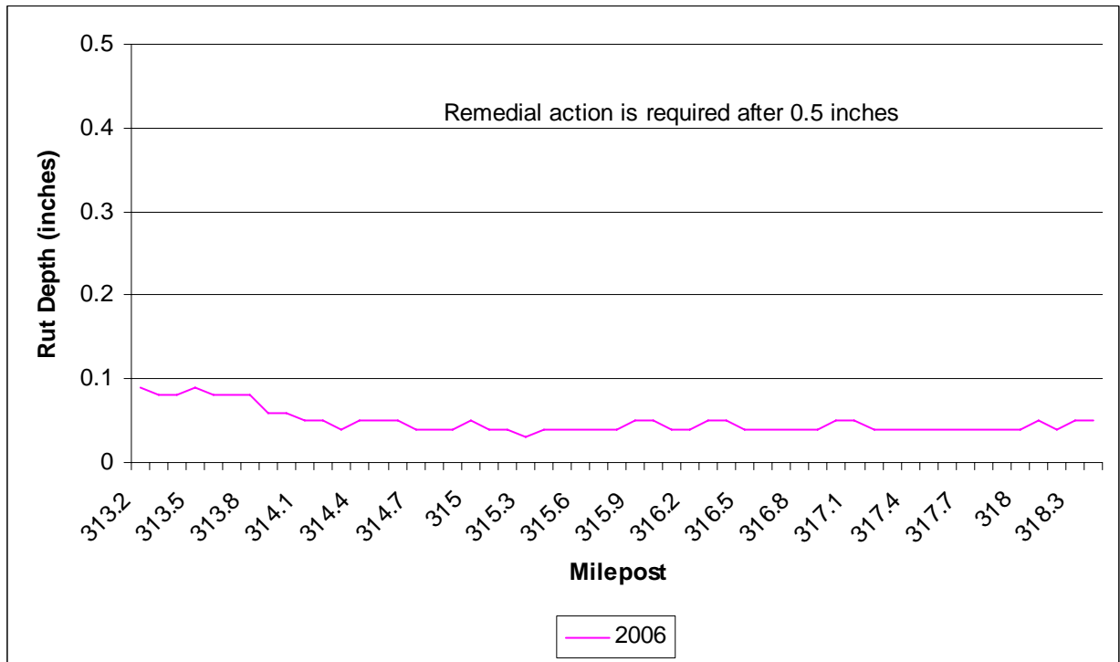
Figure 8b. PMS data for rutting on the Constitution Ave. to Garrett Rd. project (warranty).
