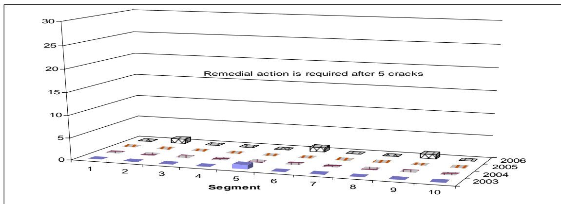
Figure 3b. PMS data for transverse cracks in the primary direction on the Stratton project (warranty).
