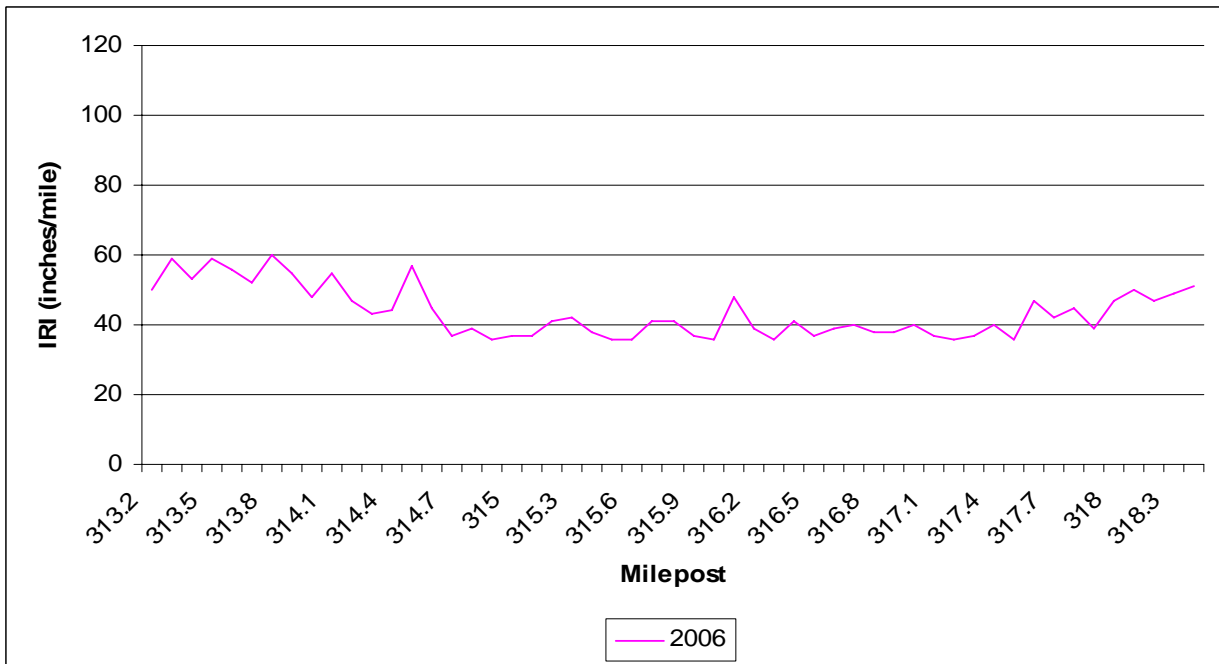
Figure 7b. PMS data for International Roughness Index on the Constitution Ave. to Garrett Rd. project (warranty).
