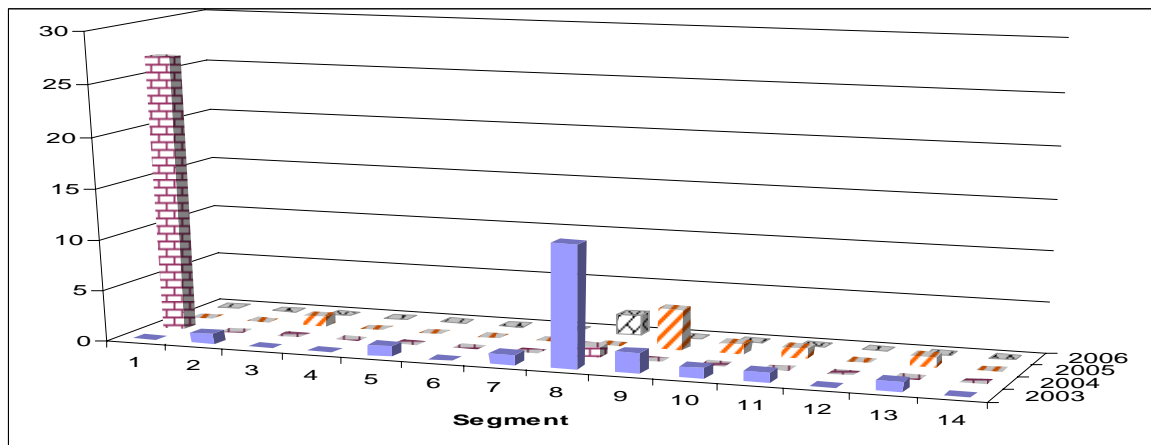
Figure 3a. PMS data for transverse cracks on the Eads project (control).
