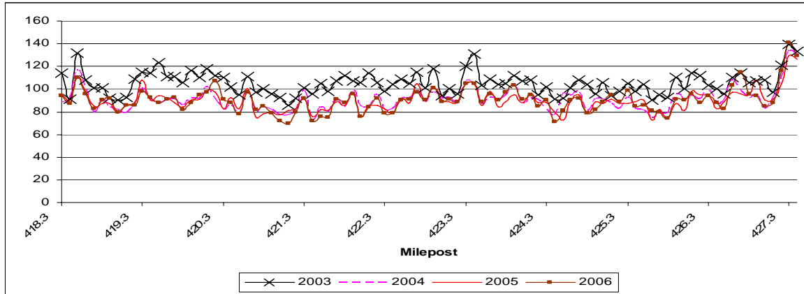
Figure 2c. PMS data for International Roughness Index data in the secondary direction on the Stratton project (warranty).
