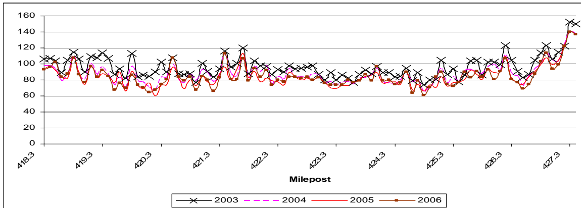
Figure 2b. PMS data for International Roughness Index data in the primary direction on the Stratton project (warranty).
