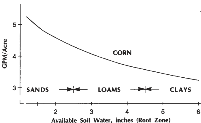
Figure 2: Net irrigation system capacities for corn in eastern Colorado.
