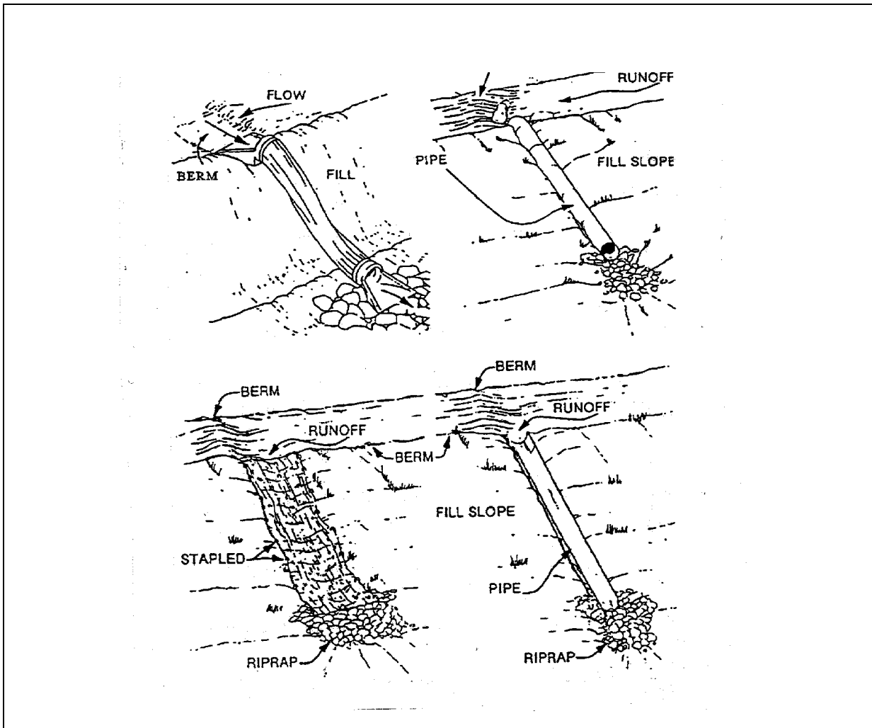
FIGURE EC 7.1 Slope Drains (CDOT ® )
