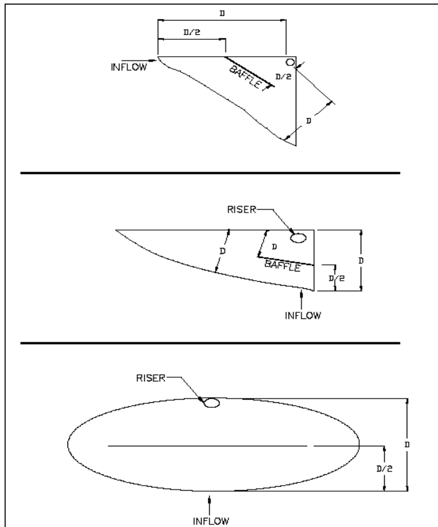
FIGURE SC 6.2 Sediment Basin Baffle Location (Adapted from UDFCD 16 )
