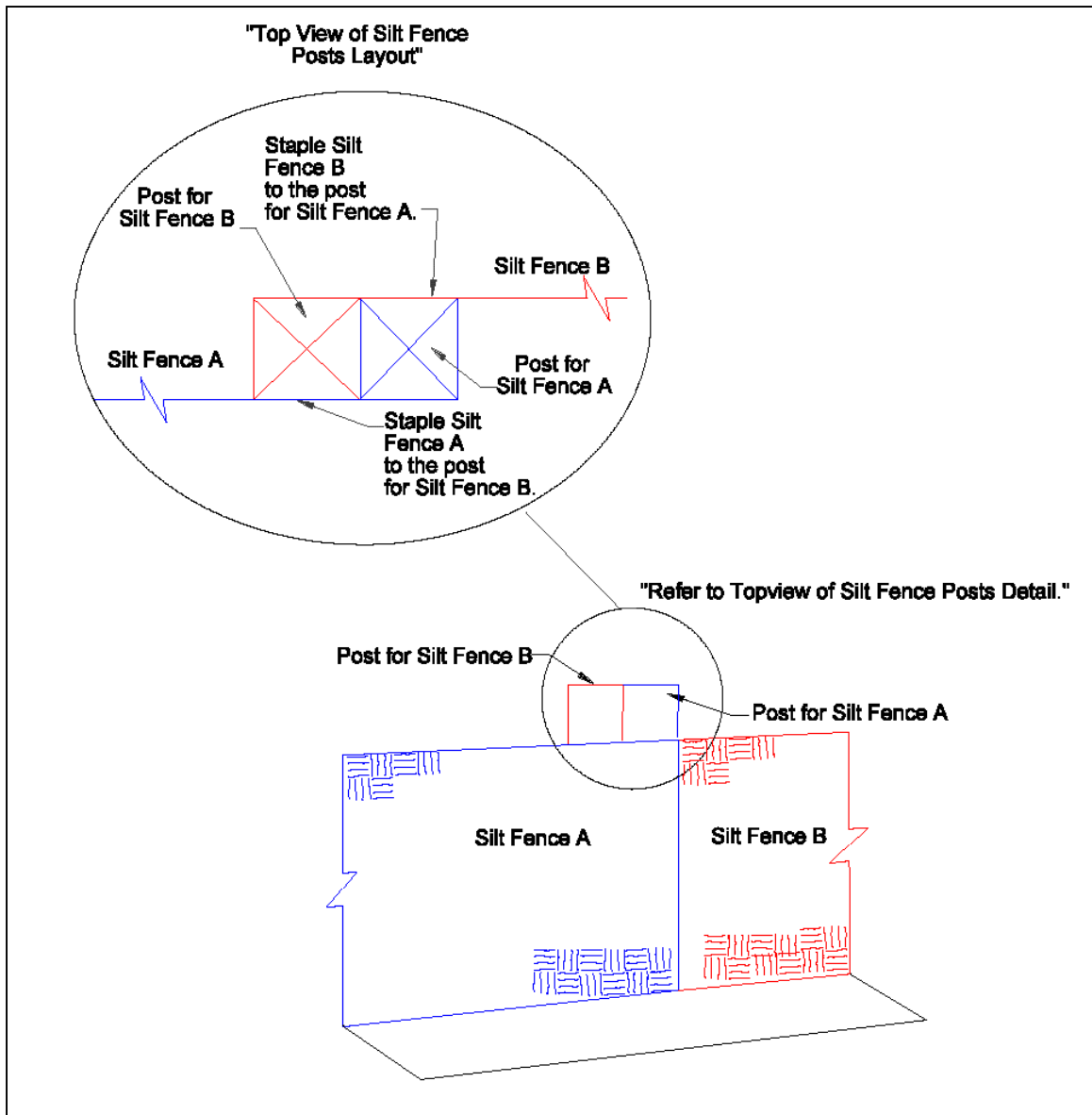
FIGURE SC 3.3 Silt Fence Joints(CDOT 18 )
