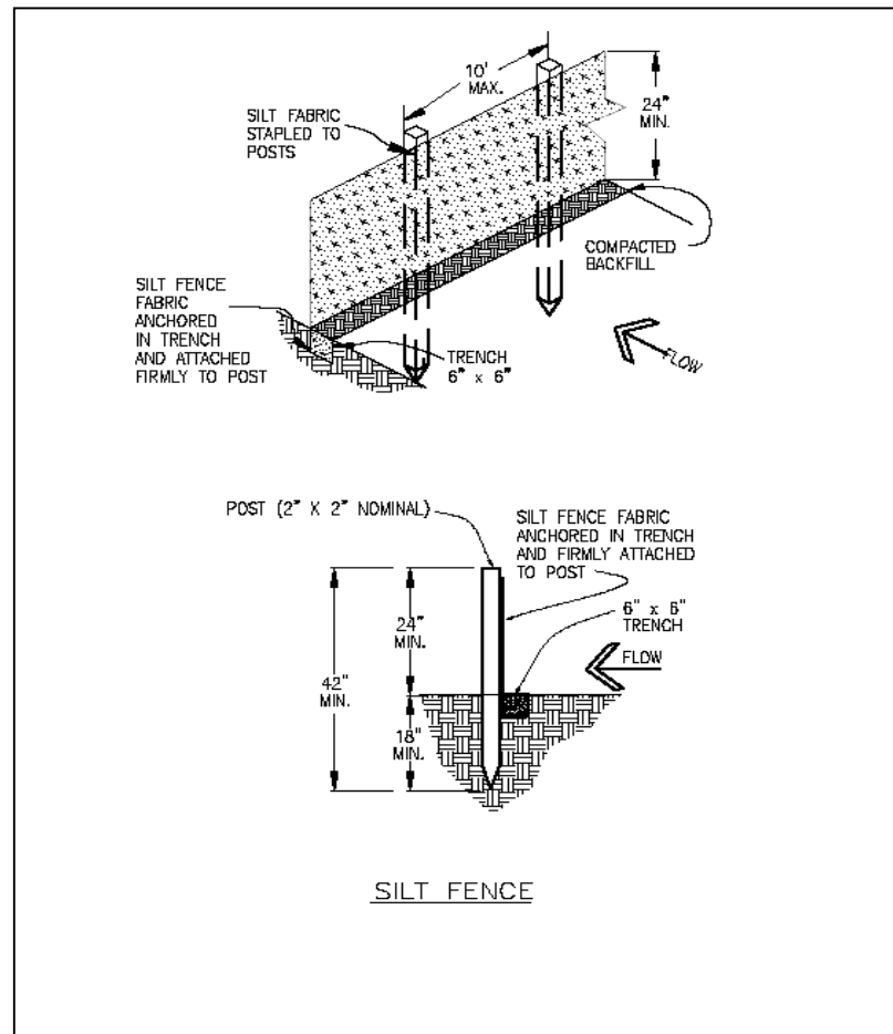
FIGURE SC 3.2 Silt Fence Installation (CDOT 18 )
