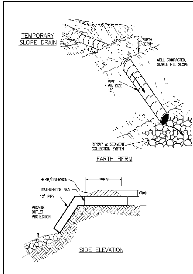
FIGURE EC 7.2 Pipe Slope Drain (CDOT 18 )
