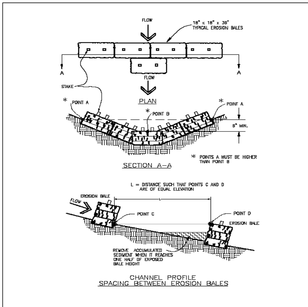
FIGURE EC 9.2 Erosion Bale Check Dams (CDOT 18 )
