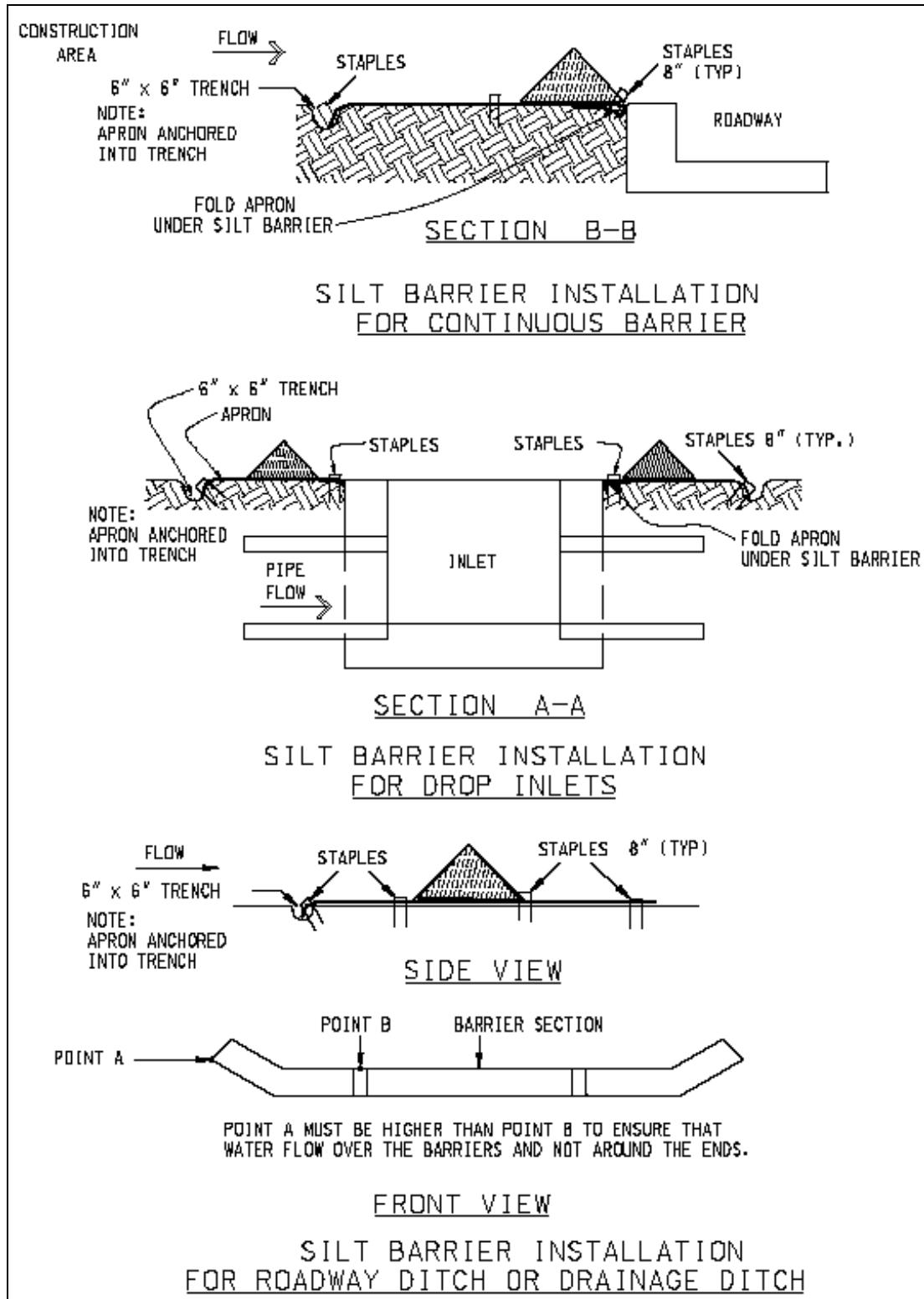
FIGURE SC 11.1 Silt Barrier Installation (CDOT 18 )
