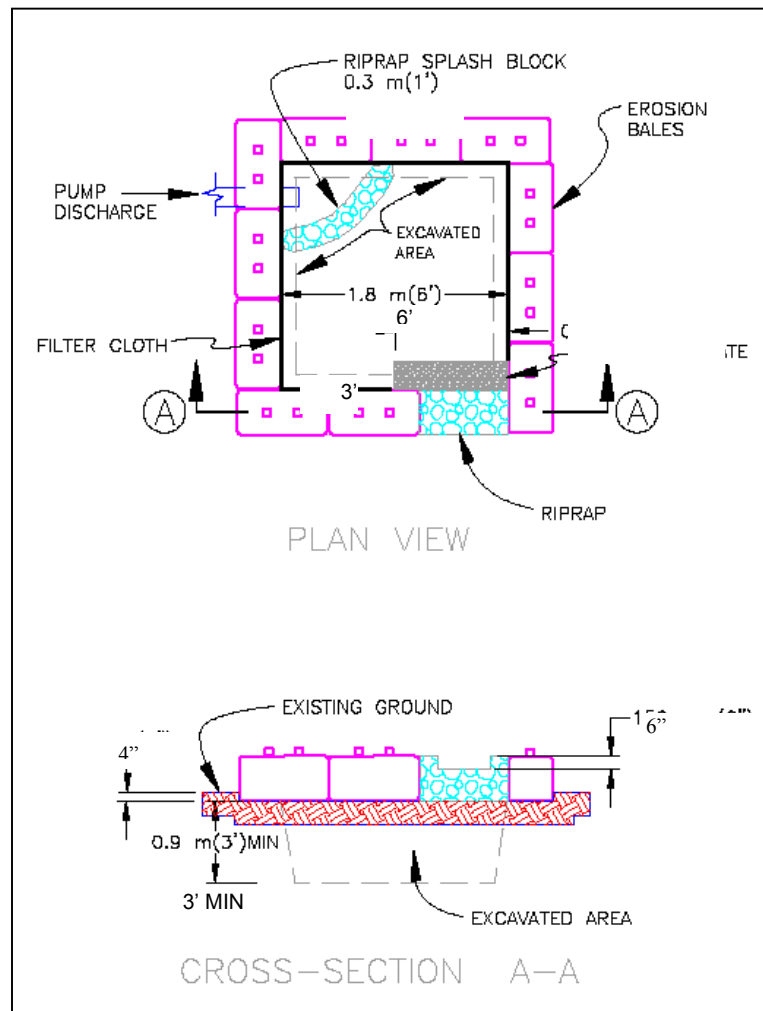
FIGURE SC 7.1 Dewatering Structure (Adapted from VEaSCH 28 )
