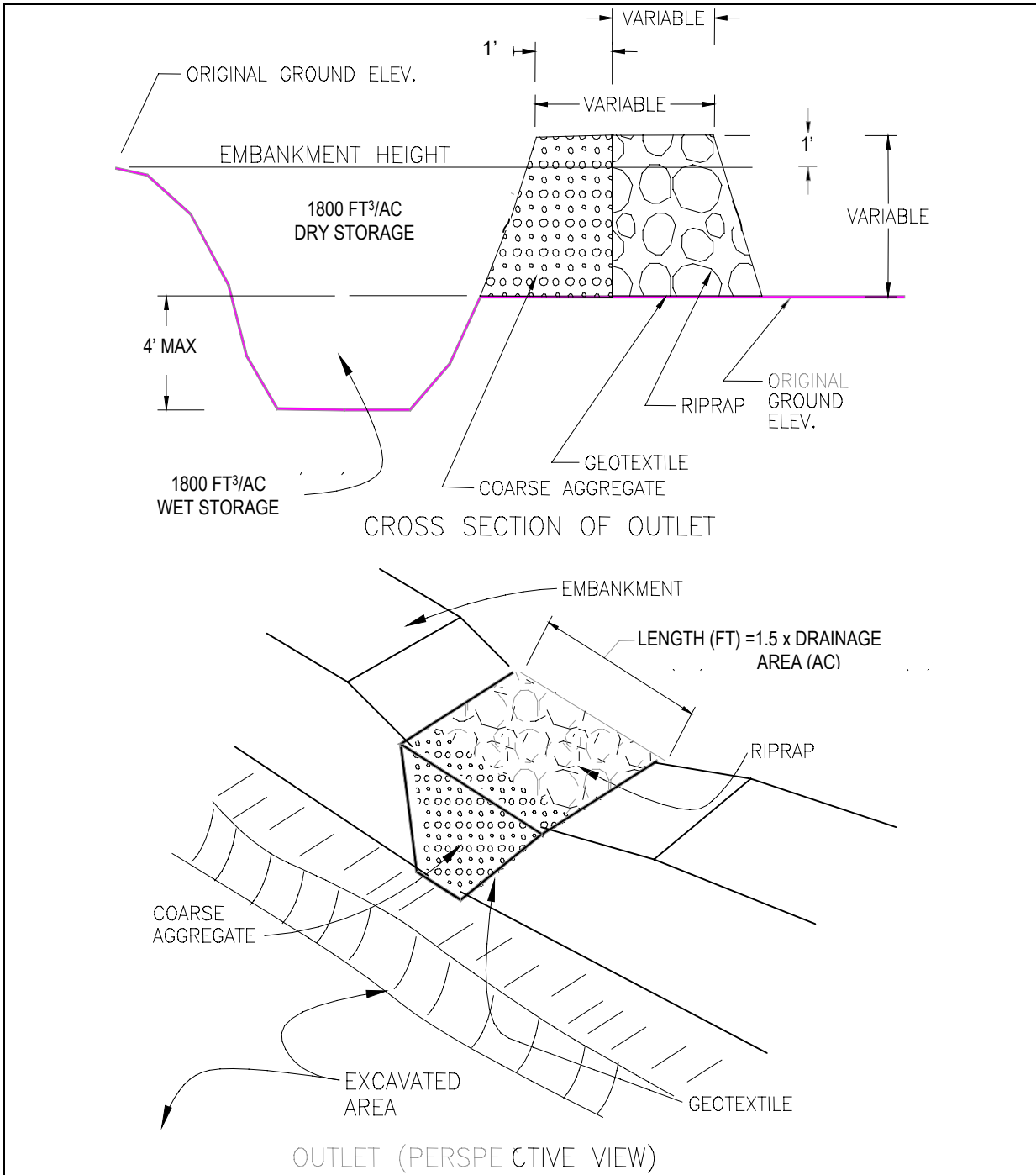
FIGURE SC 5.1 Sediment Trap (Adapted from VEaSCH 28 )
