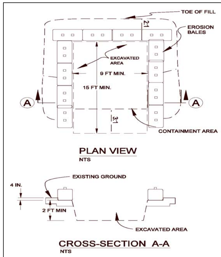
FIGURE WM1.1 Concrete Waste Management Detail
