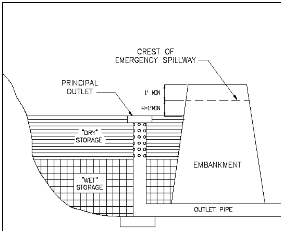
FIGURE SC 6.1 Sediment Basin (Adapted from VEaSCH 28 )
