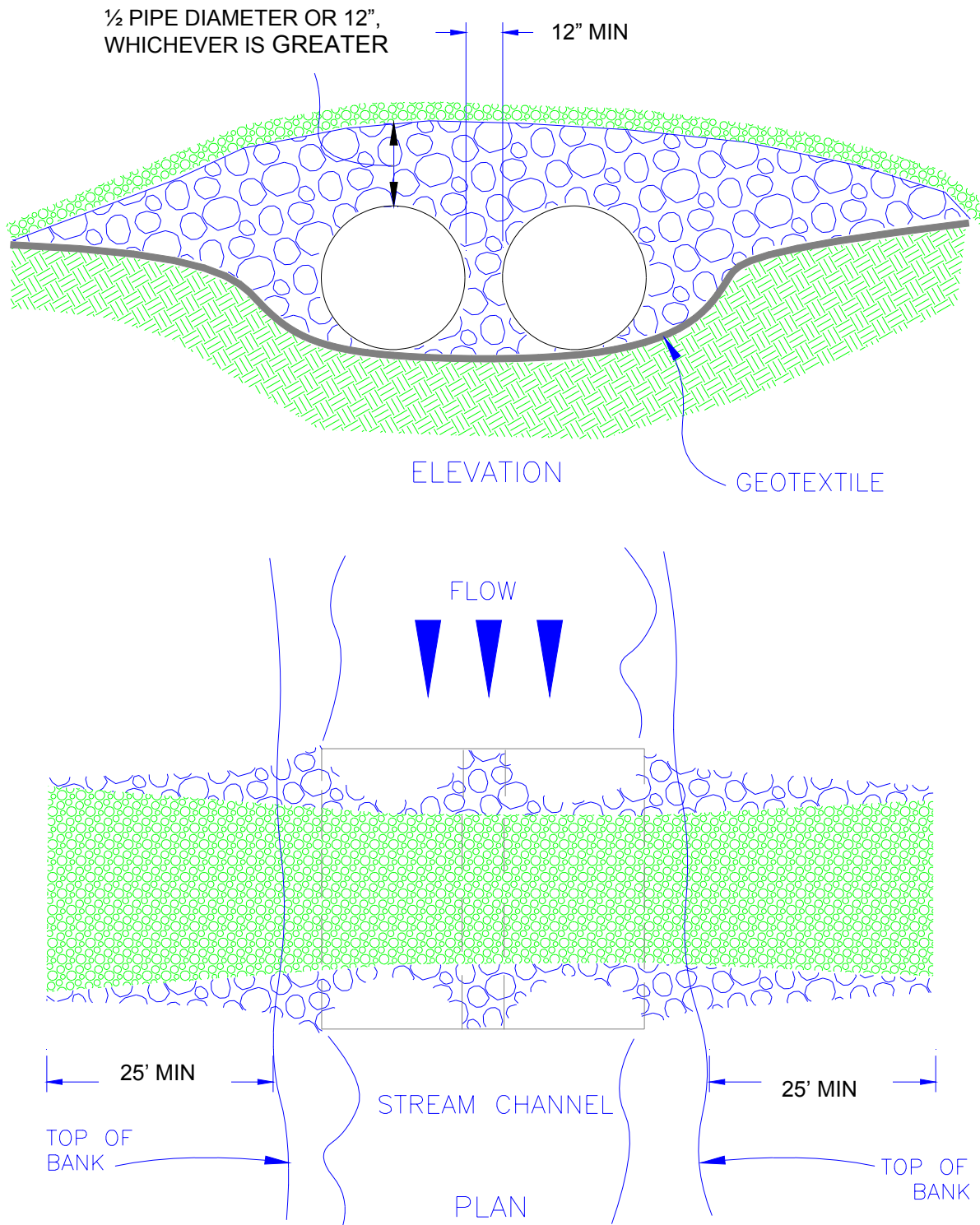
FIGURE GP 2.1 Temporary Stream Crossing
