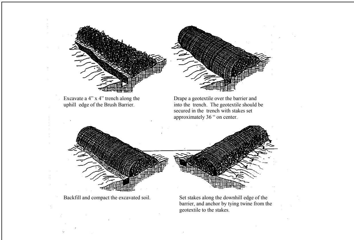
FIGURE SC 9.1 Brush Barrier (Adapted from VEaSCH 28 )
