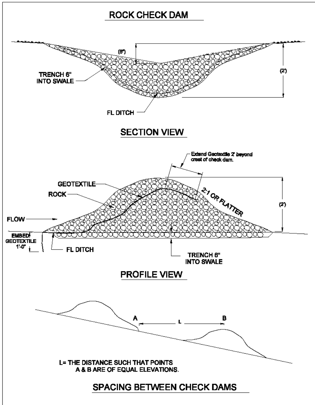
FIGURE EC 9.1 Rock Check Dam (CDOT 18 )
