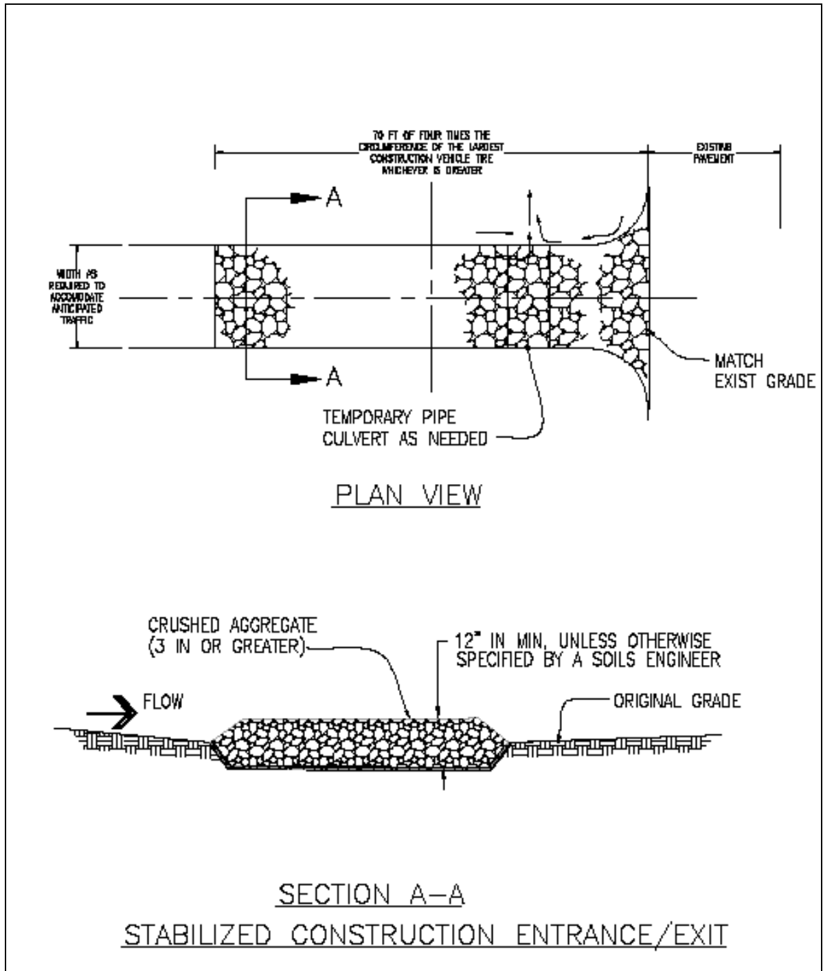
FIGURE SC 8.1 Stabilized Construction Entrance(CDOT 18 )
