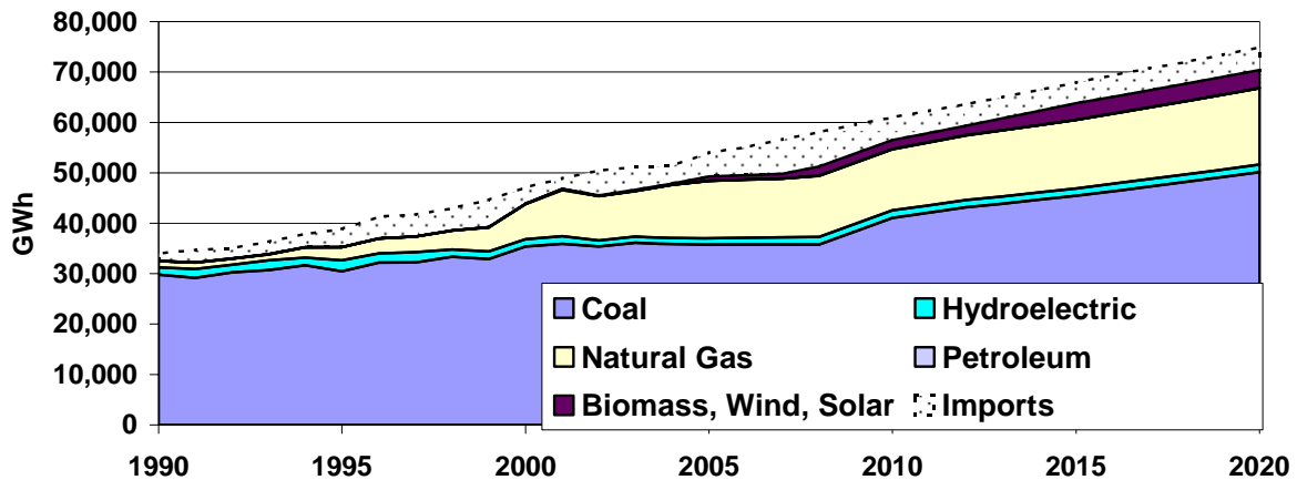
Figure A4. Electricity Generated by Colorado Power Plants plus Estimated Net Imports, 1990-2020
