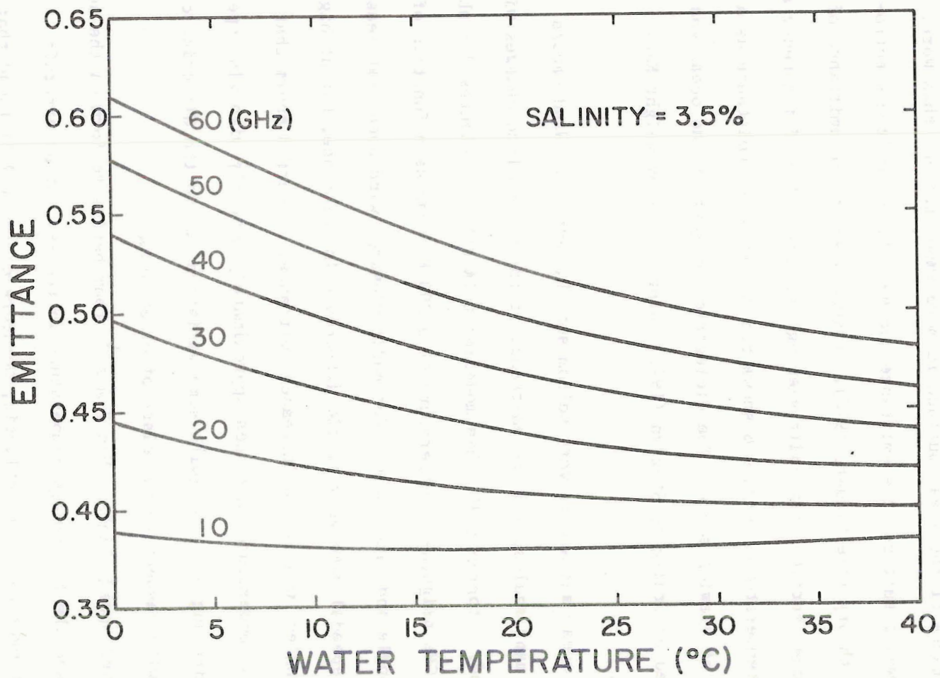
Figure 5. Nadir emittance of a smooth ocean surface as a function of surface temperature
