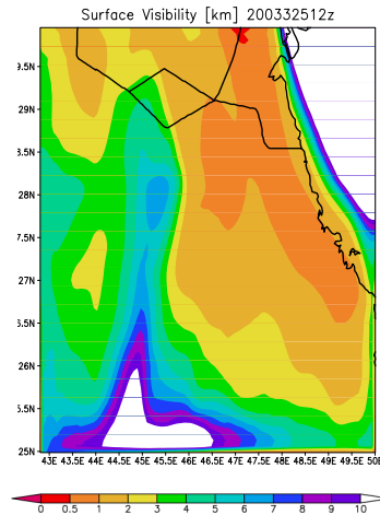
Figure 5.10: Surface visibility, grid 2: 12Z 25 March 2003.
