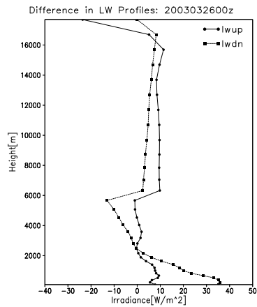
Figure 5.20: Changes in longwave radiation streams, 00Z 26 March 2003.
