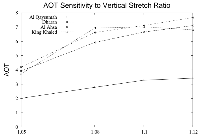
Figure 3.11: AOT sensitivity to vertical stretch ratio
