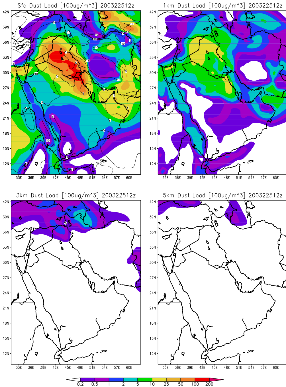
Figure 7.10: Vertical stratification of dust: 12Z 25 February 2003.
