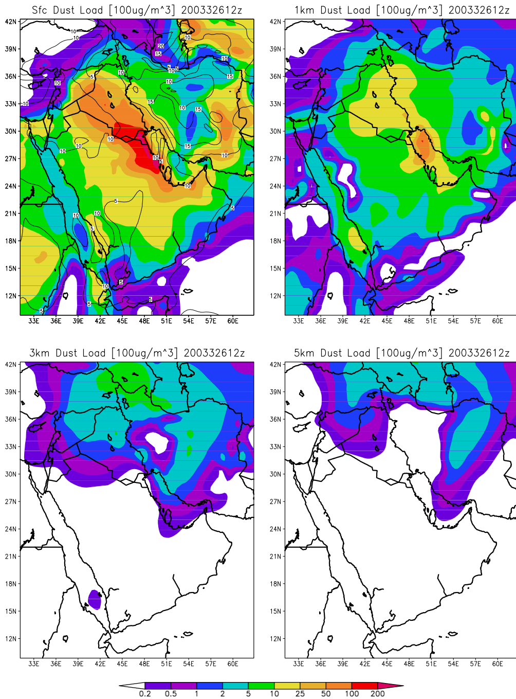
Figure 5.12: Vertical stratification of dust: 12Z 26 March 2003.
