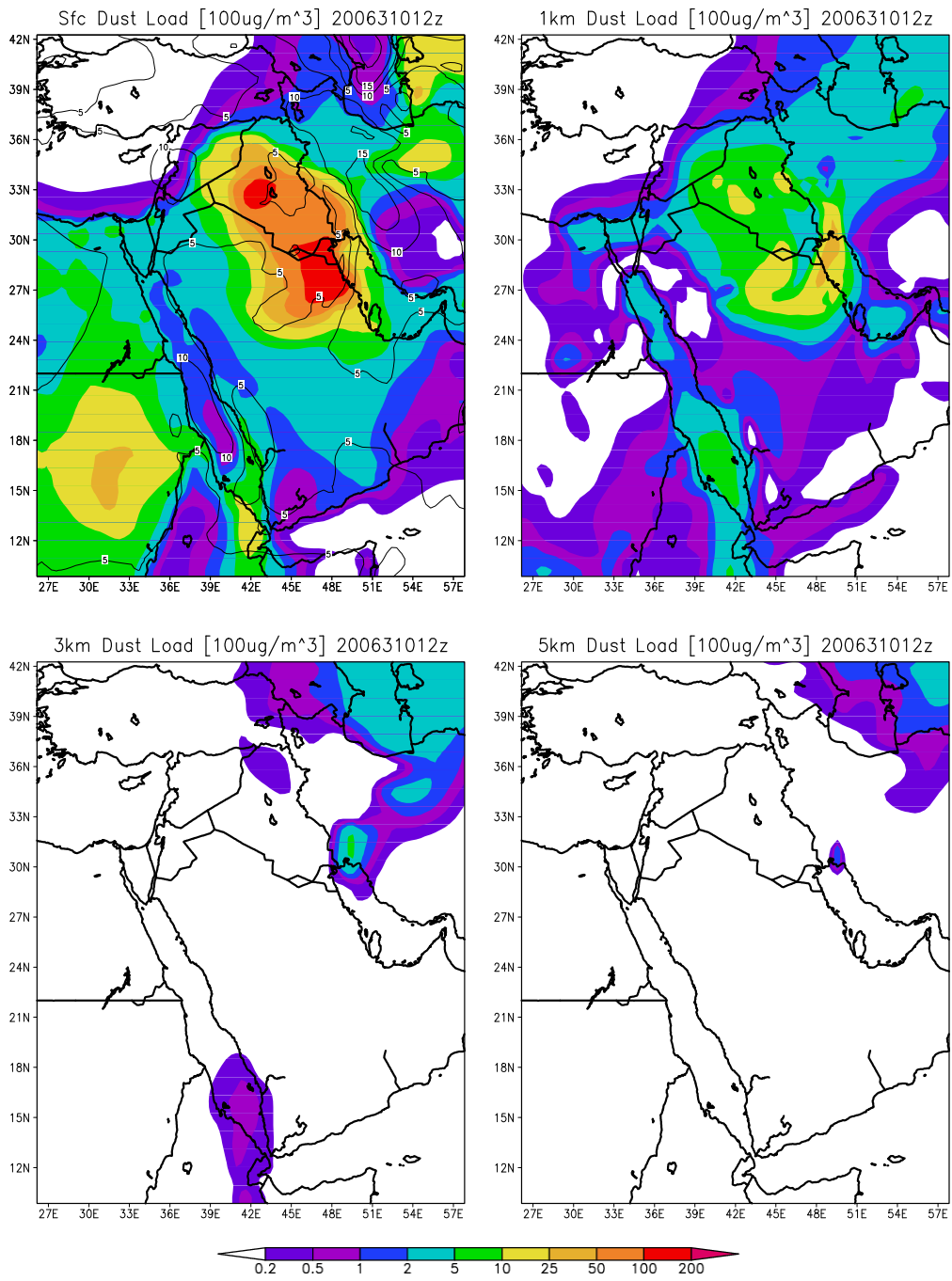
Figure 6.10: Vertical stratification of dust: 12Z 10 March 2006.
