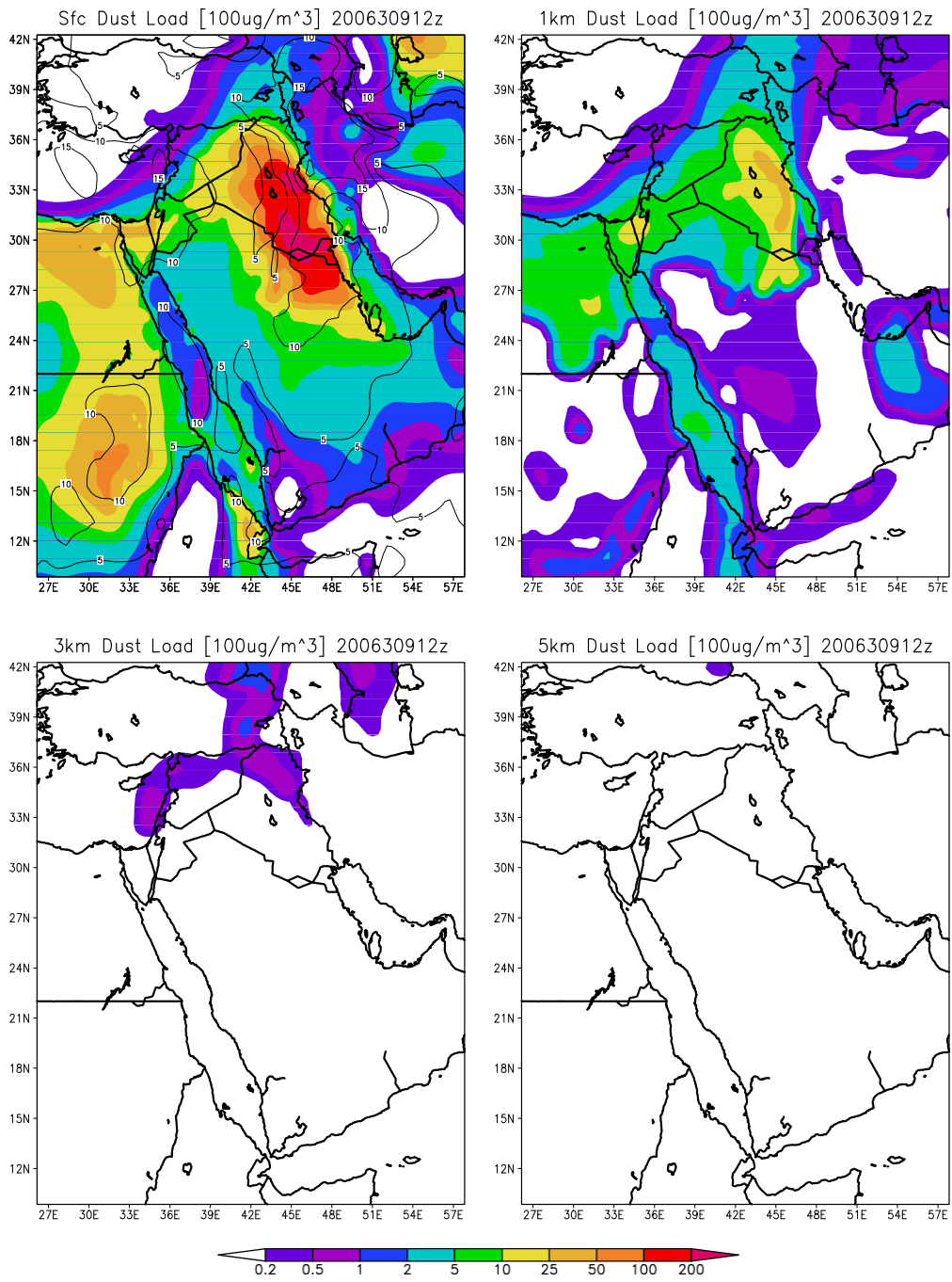
Figure 6.6: Vertical stratification of dust: 12Z 9 March 2006.
