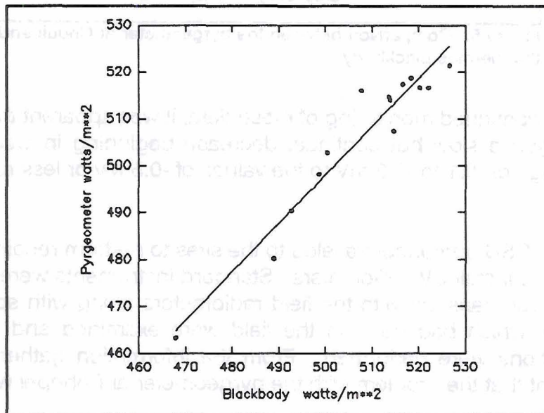
Figure 7. Comparison between the pyrometer at Pohnpei and the thermos blackbody during October, 1992.
