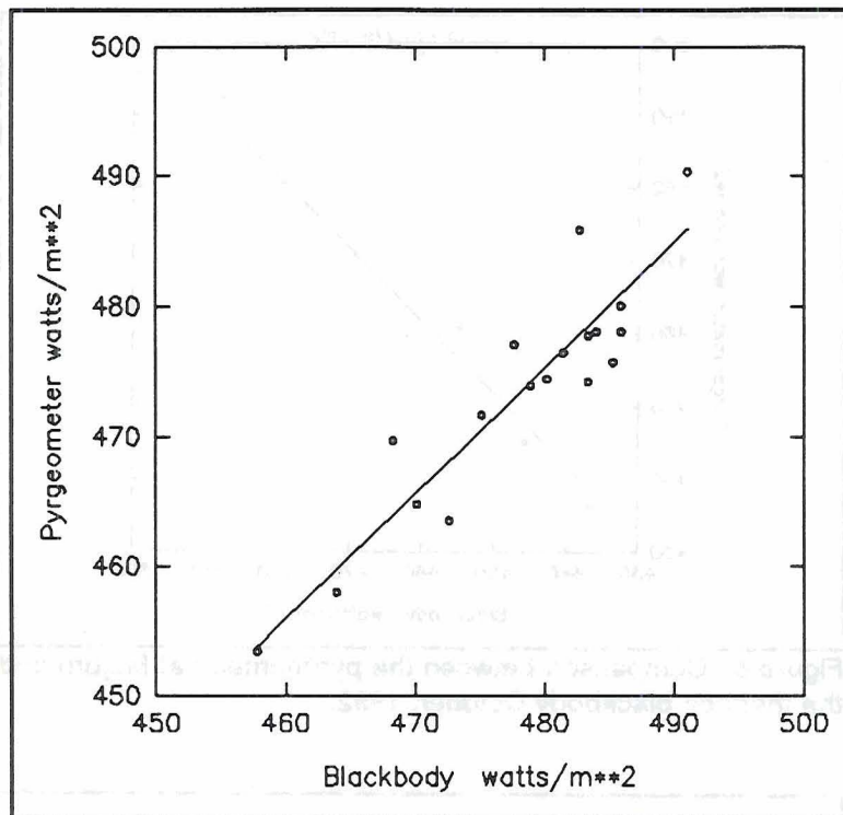
Figure 5. Comparison between the pyrgometer at Chuuk and the thermos blackbody.
