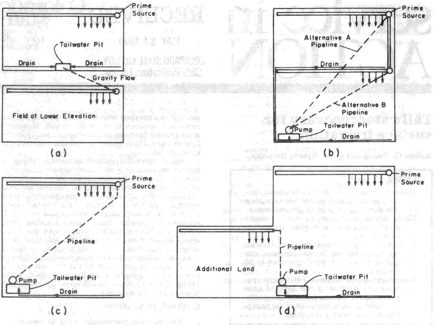
Figure 1: Alternative reuse systems: a) sequential reuse to irrigate lower-lying lands; b) alternative return reuse systems for sequential fields; c) return reuse system to the highest point in the same field; and d) return reuse system to irrigate new additional lands.
