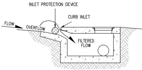
STORM DRAIN INLET PROTECTION (TYPE I) INLET PROTECTION SHALL EXTEND 12 IN. PAST EACH END OF THE INLET.
