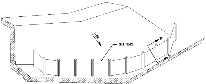
ISOMETRIC VIEW
