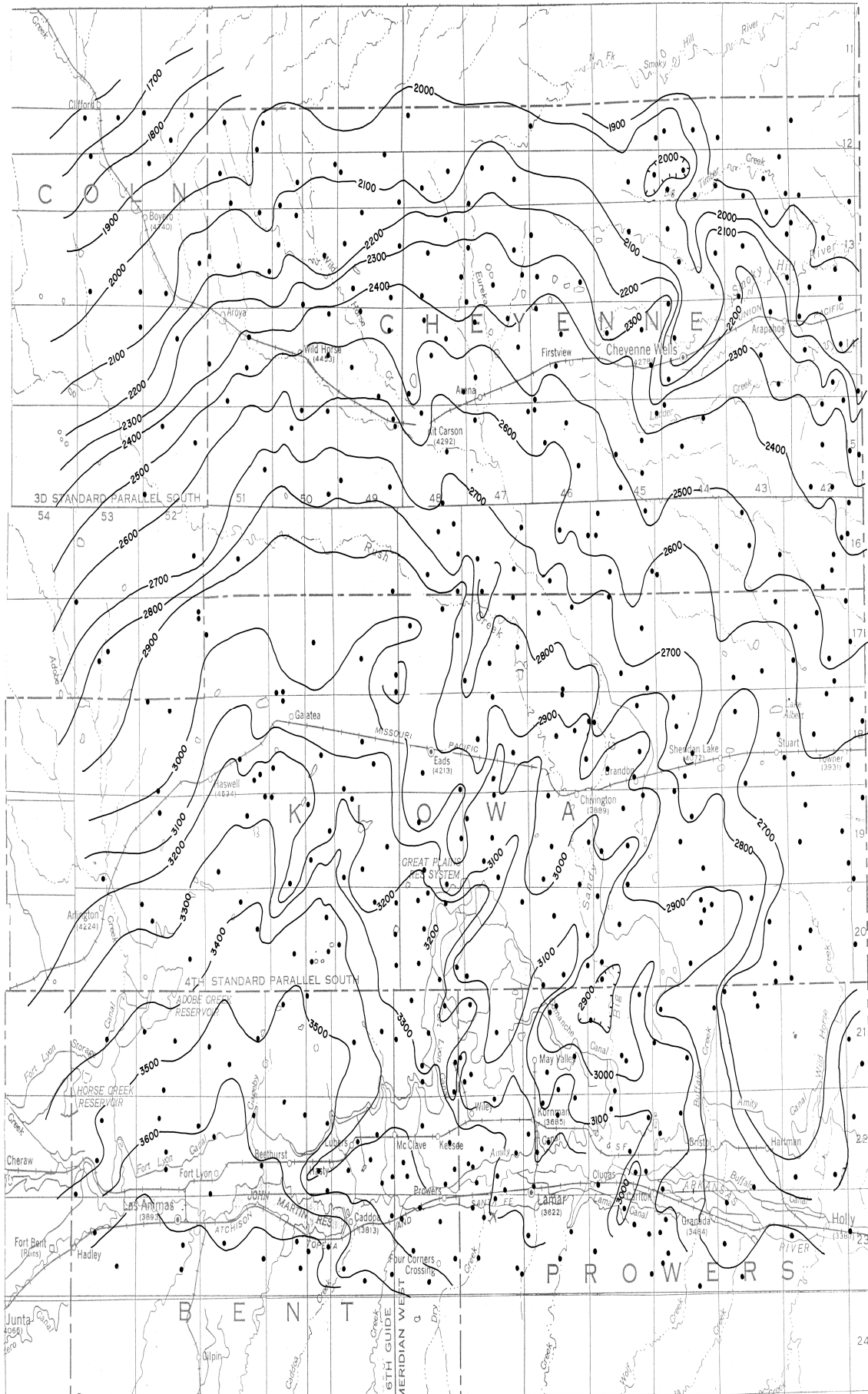
STRUCTURE CONTOUR MAP OF THE BASE OF THE DAKOTA AQUIFER IN THE CHEYENNE WELLS-ANIMAS REGION, COLORADO
