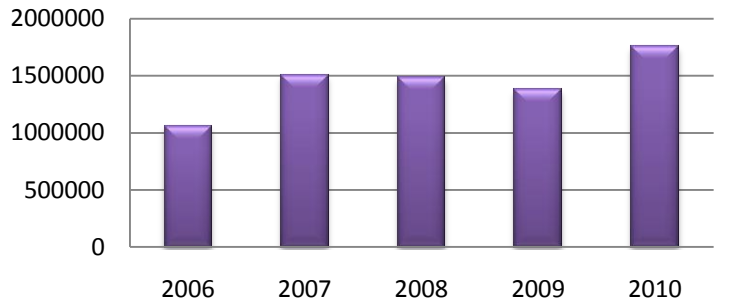
Water Division 3, Rio Grande Basin
