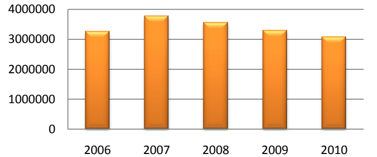
Water Division 4, Gunnison River Basin
