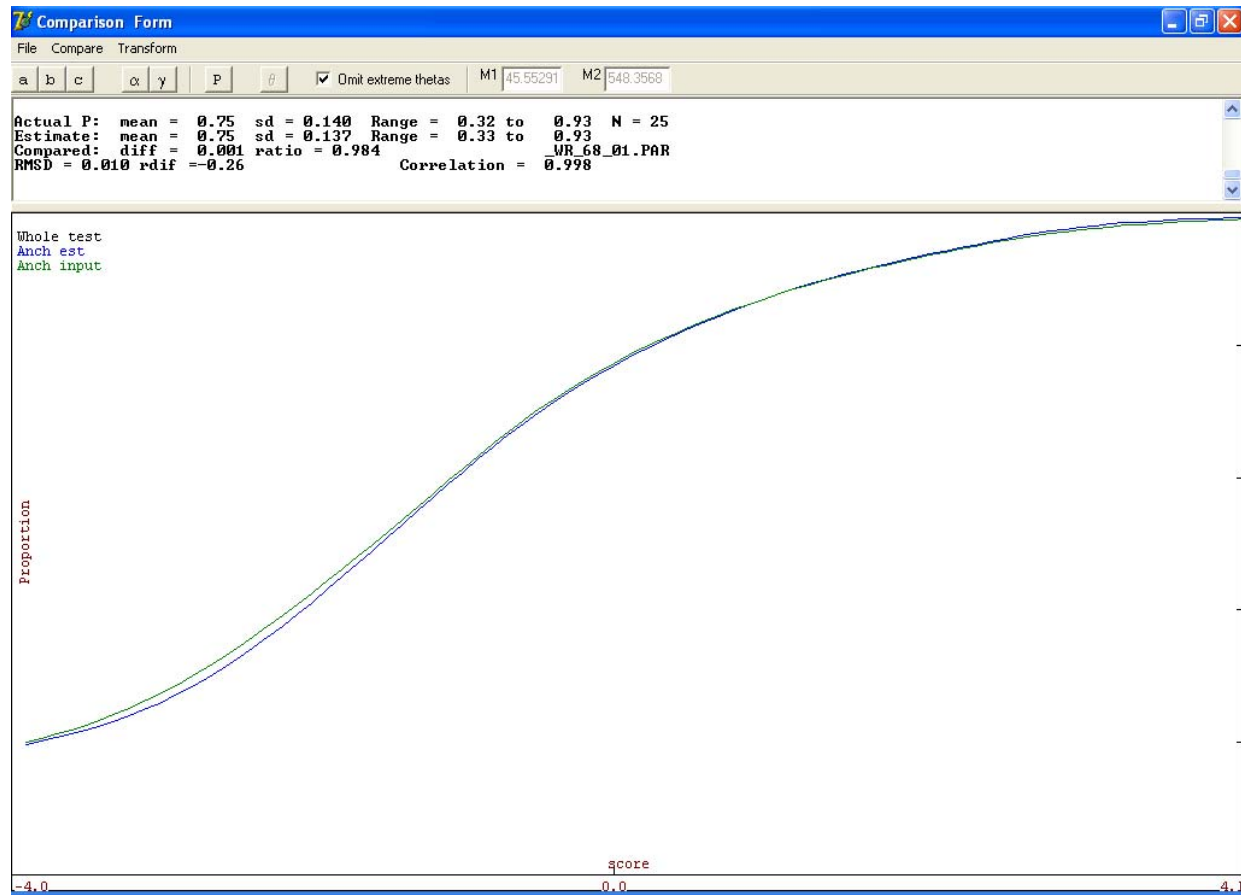
Figure 16D. Stocking & Lord Test Characteristic Curves, Grade Span 3: 6–8 Writing
