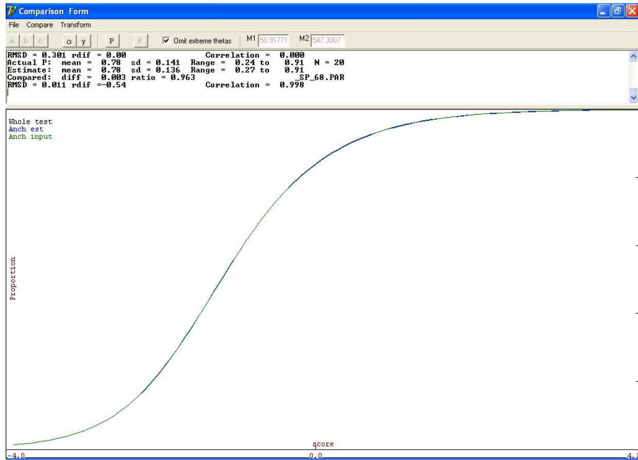
Figure 13D. Stocking & Lord Test Characteristic Curves, Grade Span 3: 6–8 Speaking
