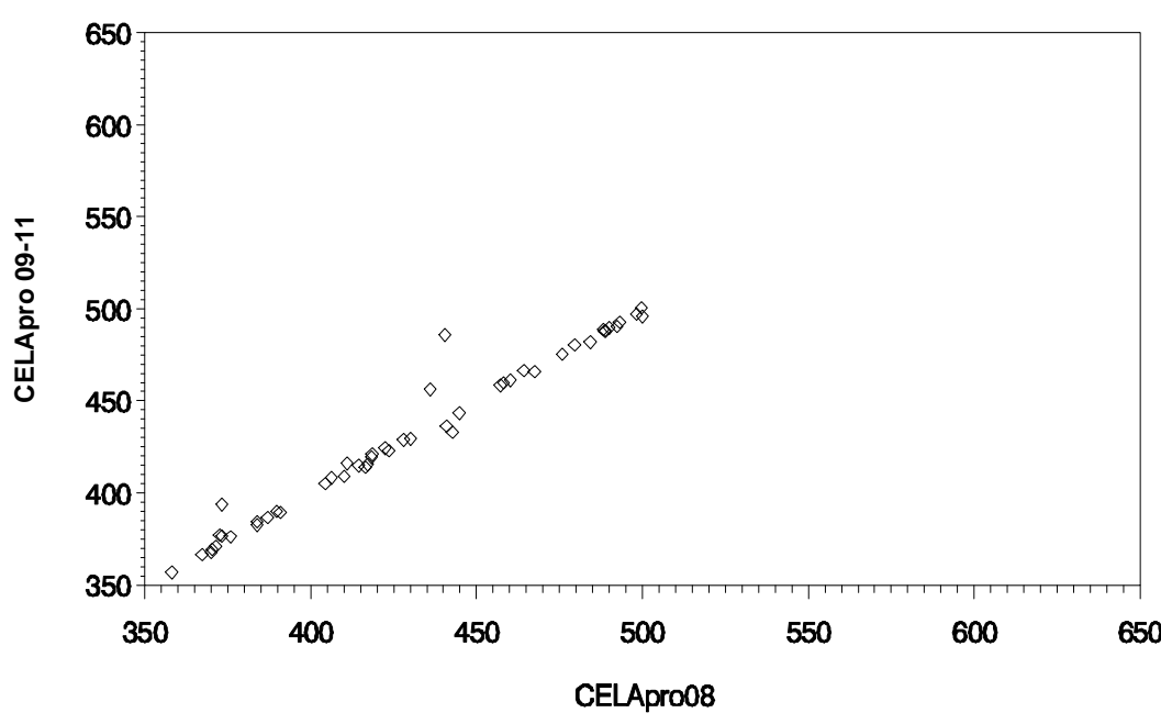
Figure 12. 'B' Anchor Parameters for Comprehension Items CELApro 08 vs. CELApro 09–11
