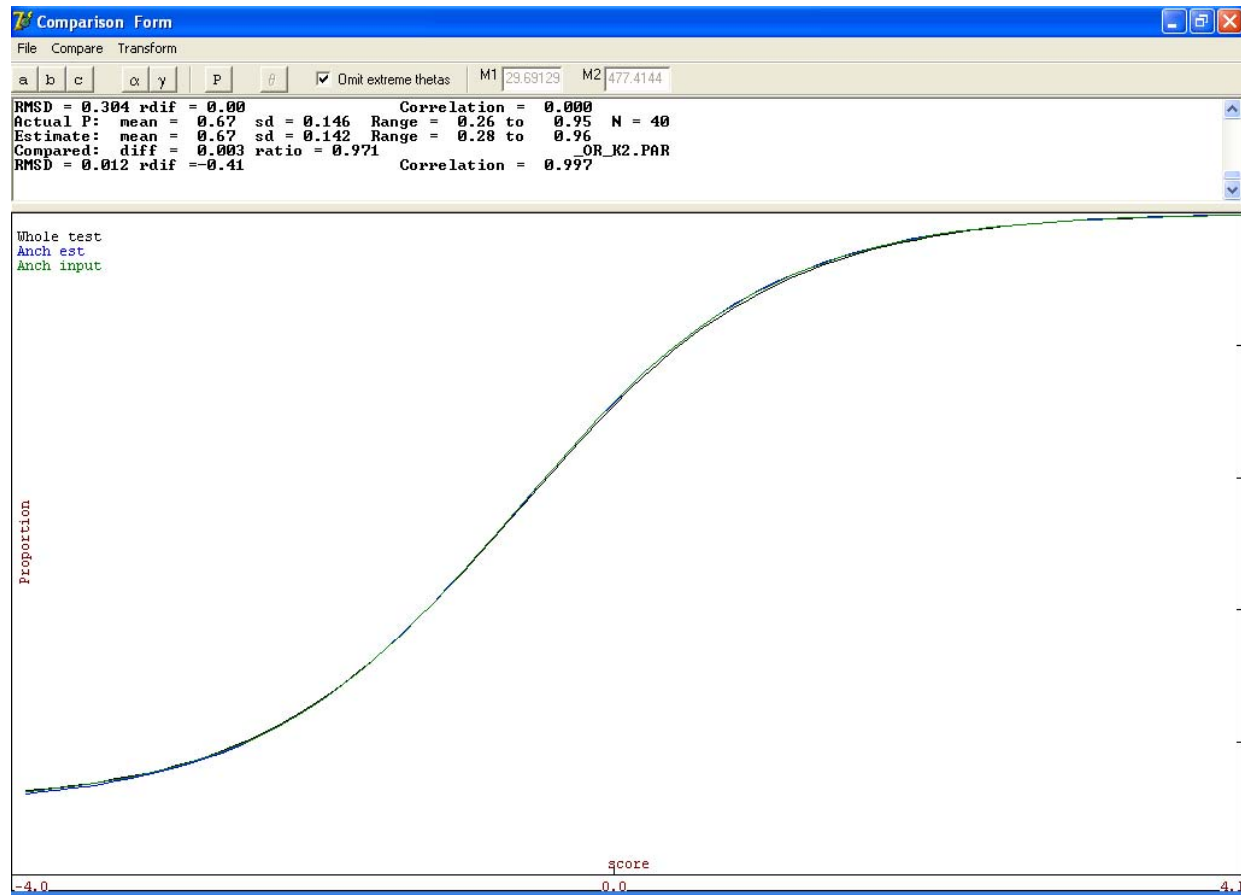
Figure 6D. Stocking & Lord Test Characteristic Curves, Grade Span 1: K–2 Oral
