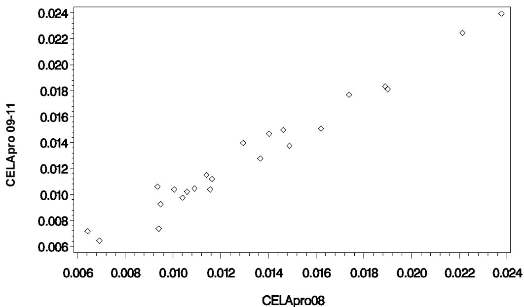
Figure 43. 'A' Anchor Items for Oral SR Items CELApro 08 vs. CELApro 09–11
