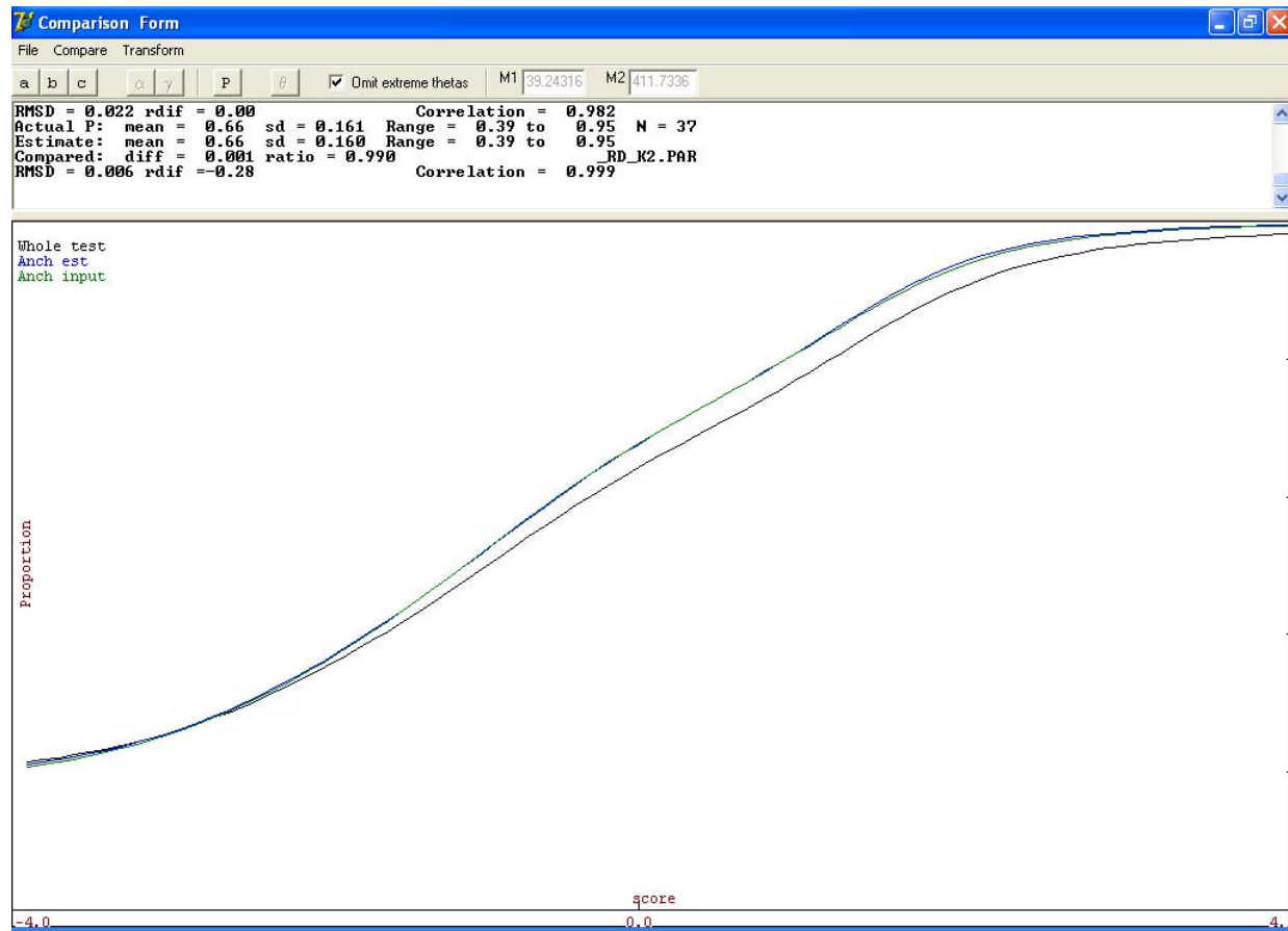
Figure 3D. Stocking & Lord Test Characteristic Curves, Grade Span 1: K–2 Reading
