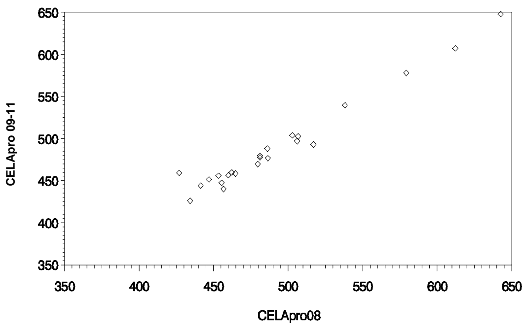
Figure 44. 'B' Anchor Items for Oral SR Items CELApro 08 vs. CELApro 09–11
