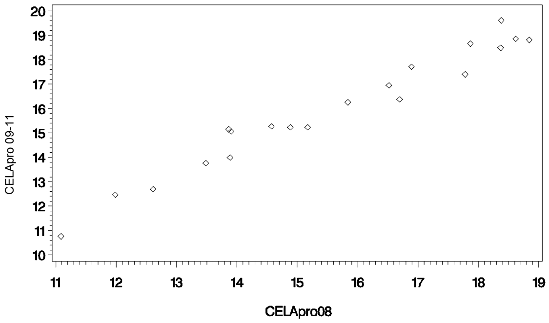
Figure 18. 'B' Anchor Parameters for Speaking Items CELApro 08 vs. 09–11
