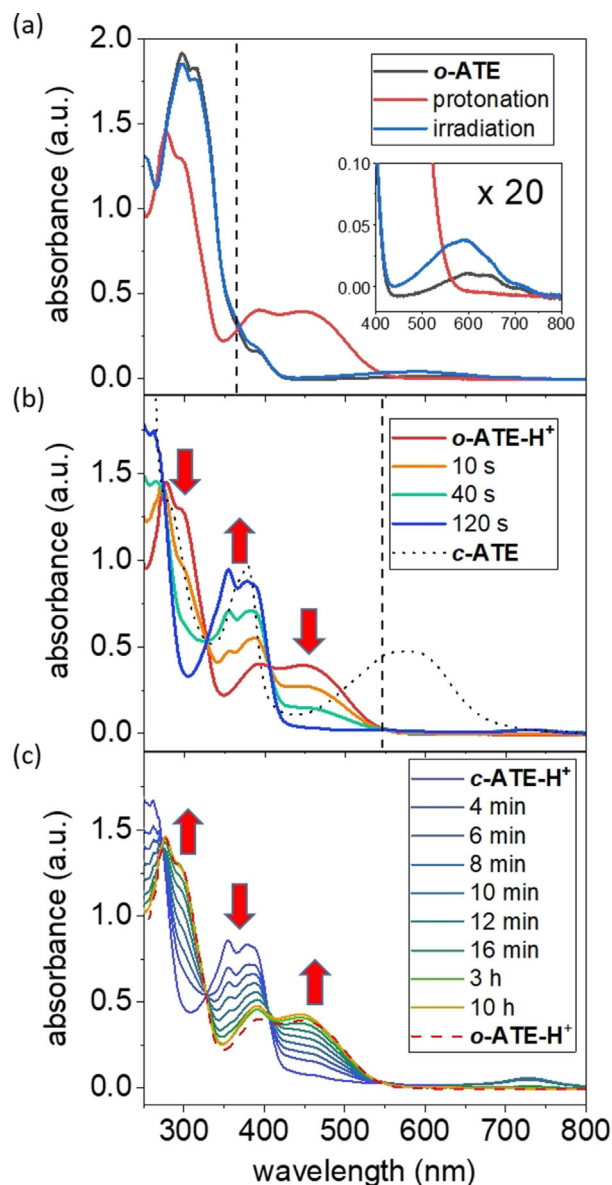
Figure 2. UV/Vis absorption spectra of (a) o -ATE (5.0 \times 10^{-5} M in cyclohexane, black) either after irradiation at 365 nm for 5 min (blue) or after addition of TFA (3.0 \times 10^{-2} M) to form o -ATE- H^+ (red). (b) o -ATE- H^+ (red) upon irradiation at 546 nm for 2 min at -30^\circ\text{C} to yield c -ATE- H^+ (blue) and subsequent addition of excess triethylamine (9.0 \times 10^{-2} M) to form c -ATE (black). (c) Thermal ring-opening of c -ATE- H^+ to o -ATE- H^+ at room temperature. Irradiation wavelengths are indicated by dash lines.
